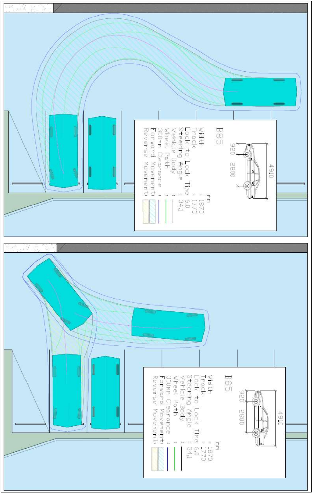
FIGURE 4.11 – SWEEP PATH OF B85 VEHICLES (MANOEUVRING)
