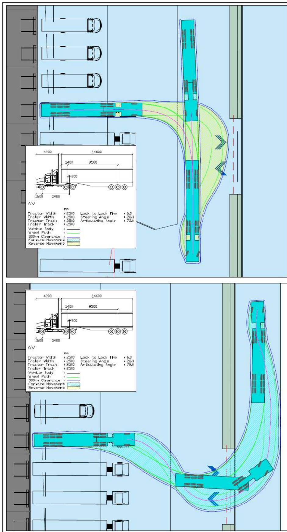
FIGURE 6.4 – VEHICLE SWEEP PATHS (ARTICULATED VEHICLE)
