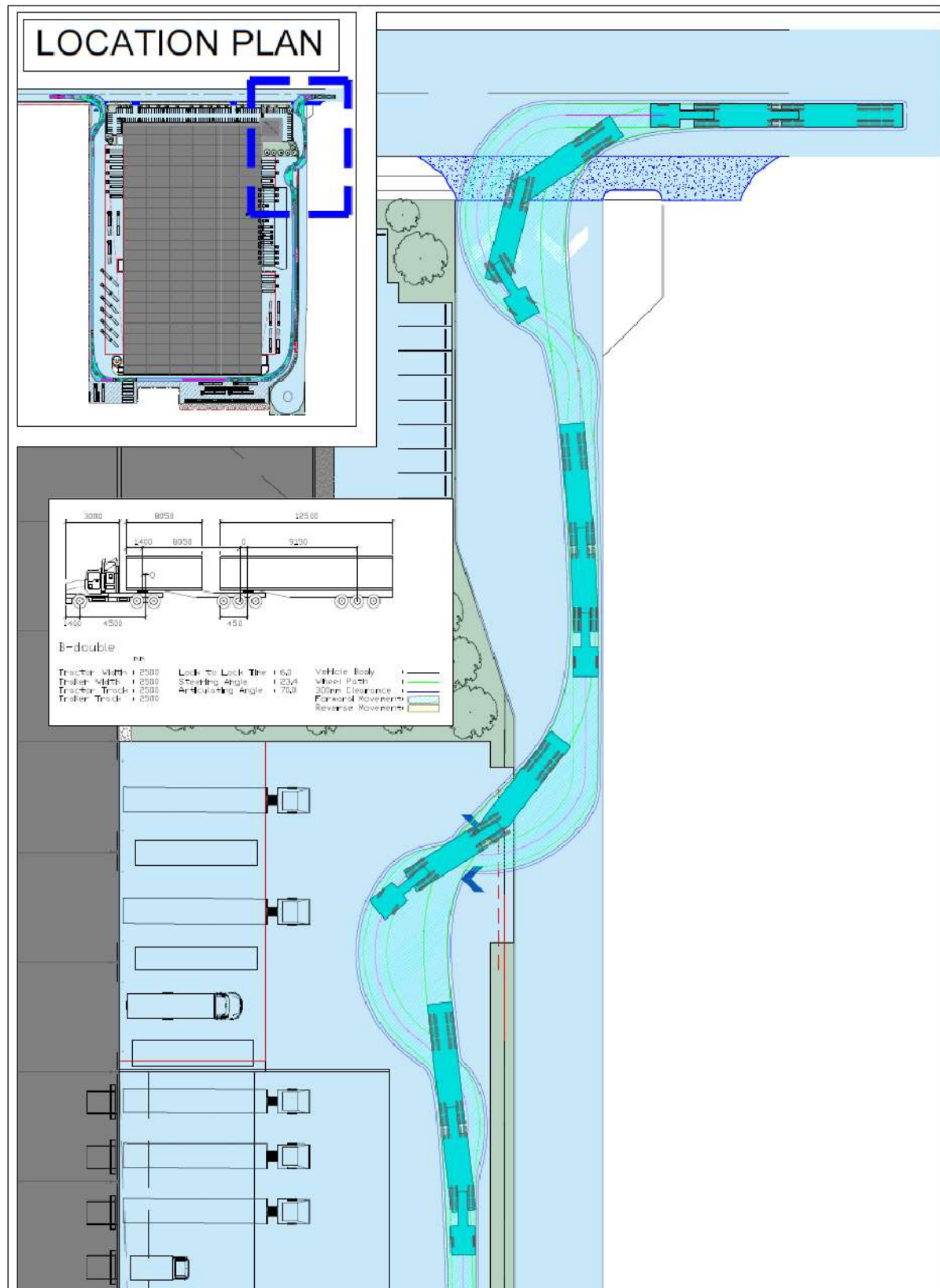
FIGURE 6.6 – VEHICLE SWEEP PATH (B-DOUBLE VEHICLE)
