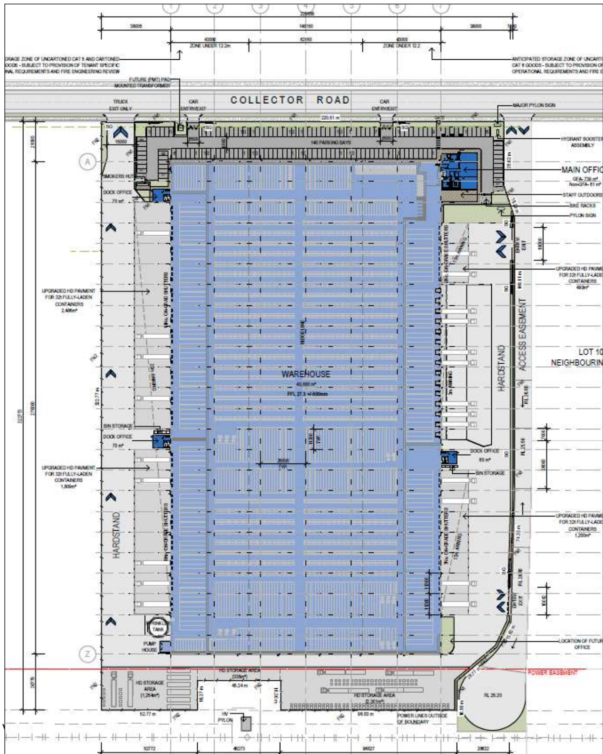
FIGURE 3.1 – PROPOSED SITE PLAN
