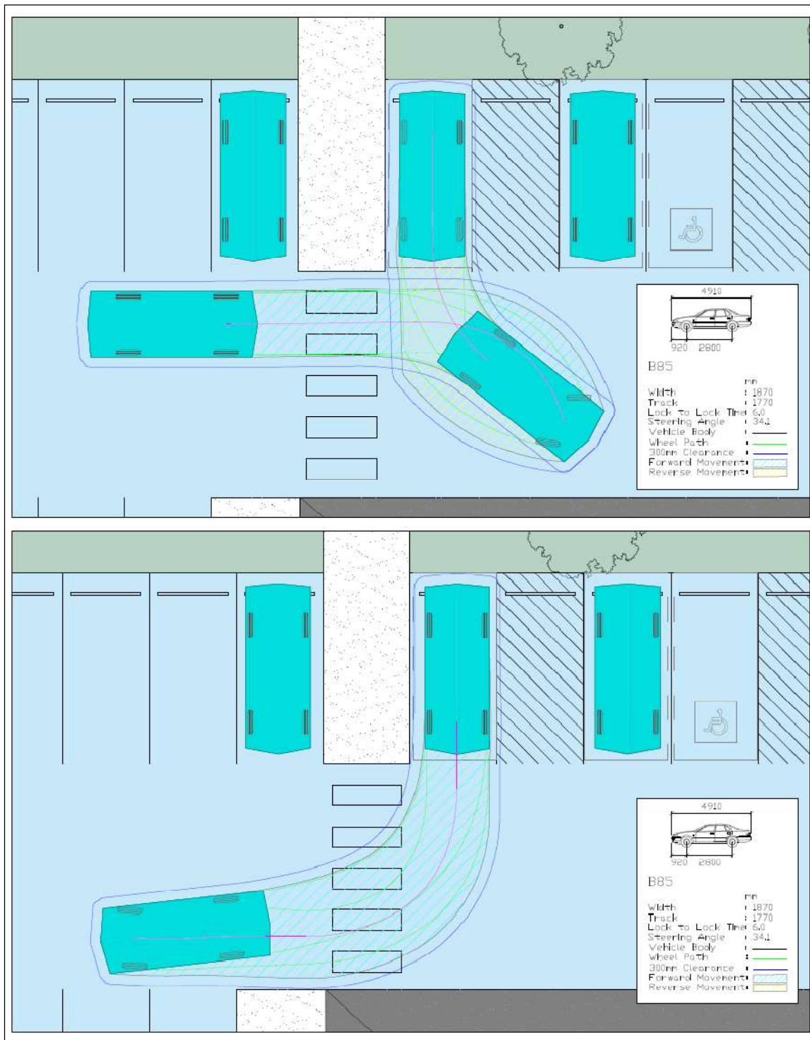
FIGURE 4.8 – SWEEP PATH OF B85 VEHICLES (MANOEUVRING)
