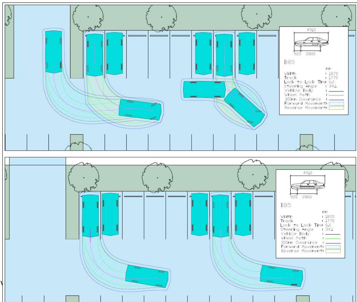
FIGURE 4.7 – SWEEP PATH OF B85 VEHICLES (MANOEUVRING)
