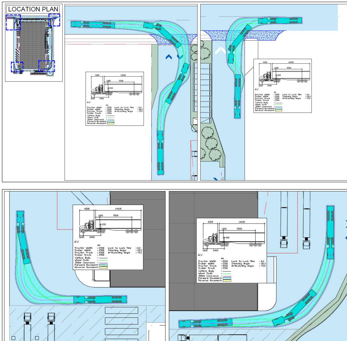
FIGURE 6.1 –SWEEP PATHS FOR ARTICULATED VEHICLE AT VEHICLE CROSSOVERS
