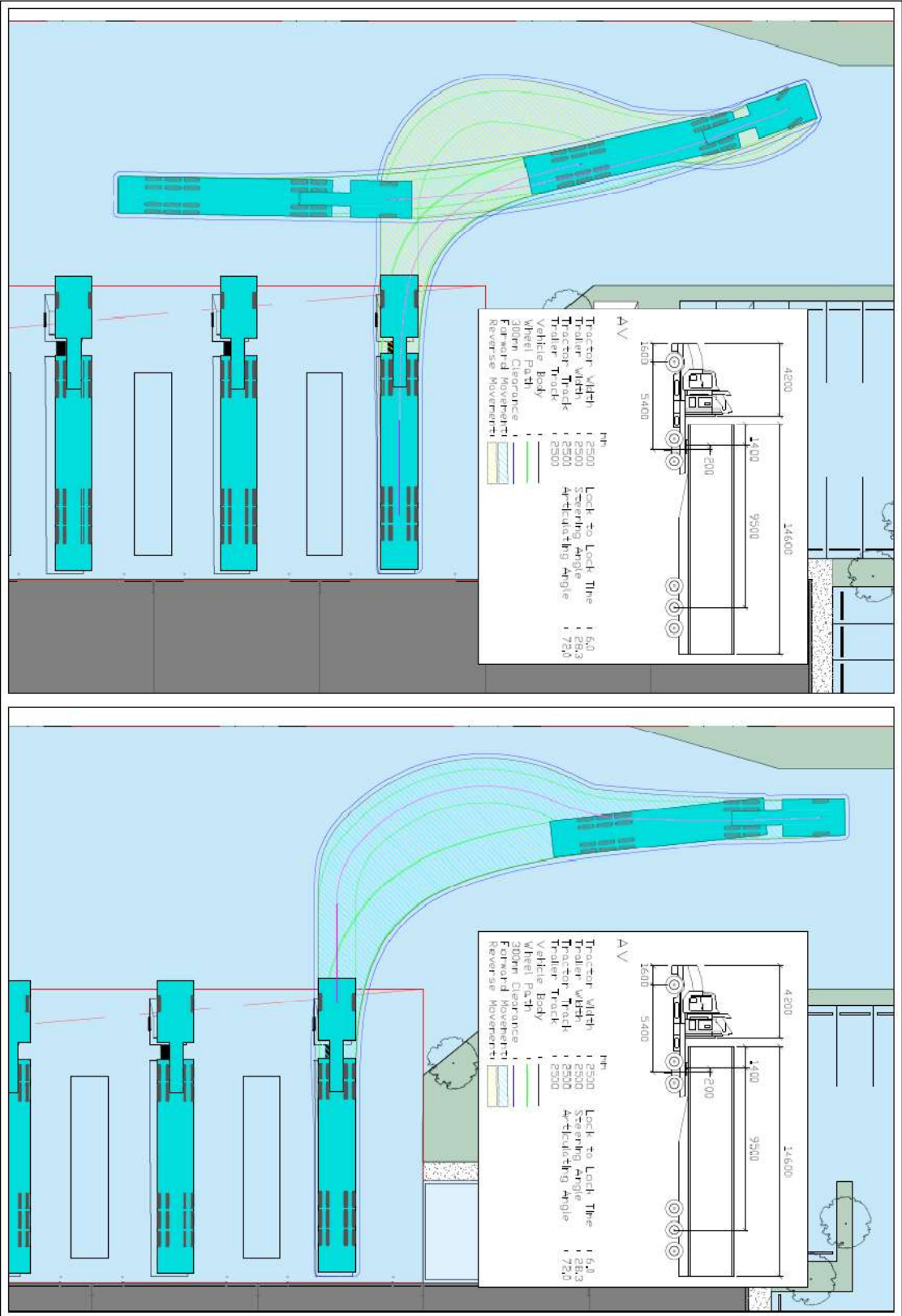
FIGURE 6.5 – VEHICLE SWEEP PATH (ARTICULATED VEHICLE)
