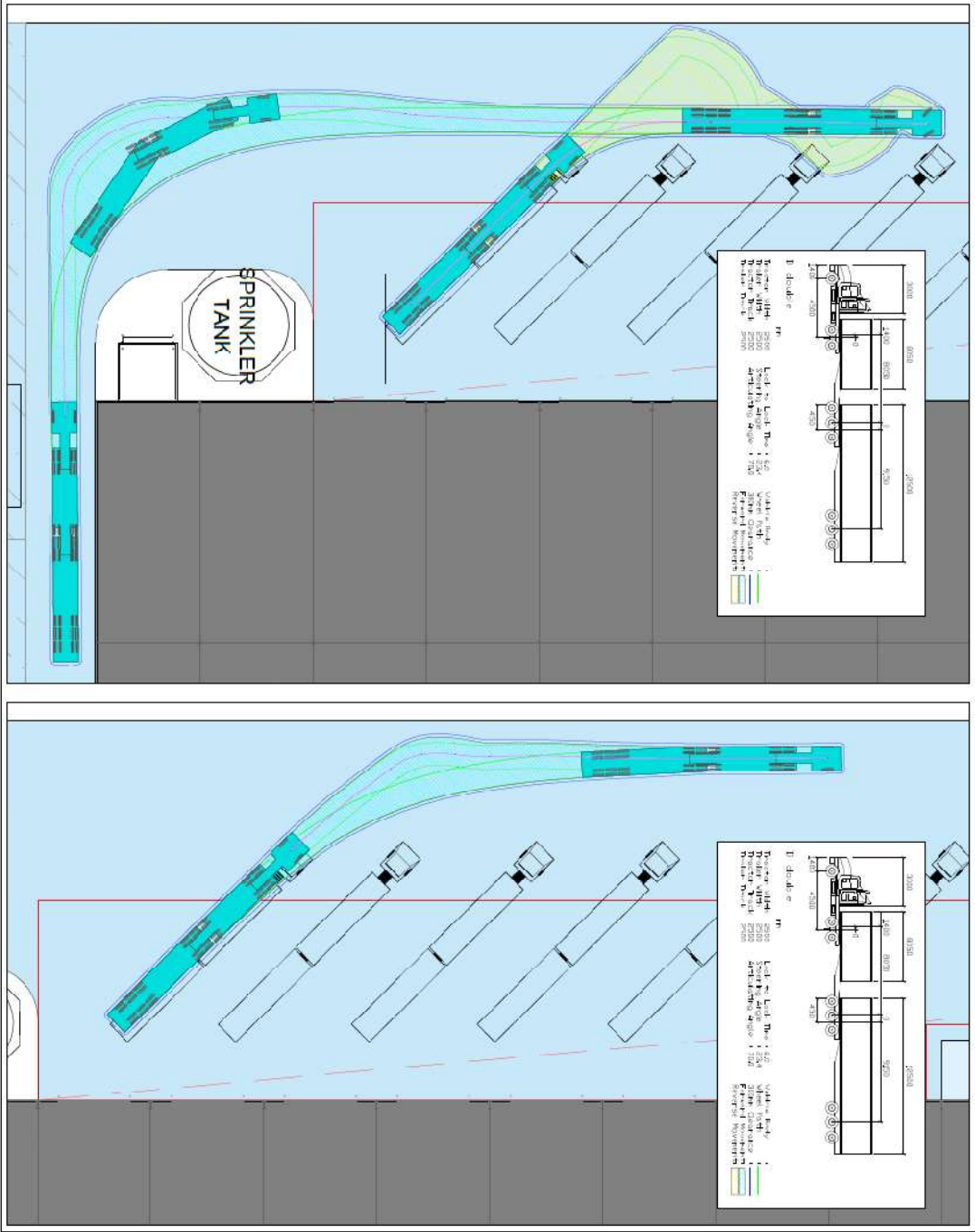
FIGURE 6.11 - VEHICLE SWEPT PATH (B-DOUBLE VEHICLE)
