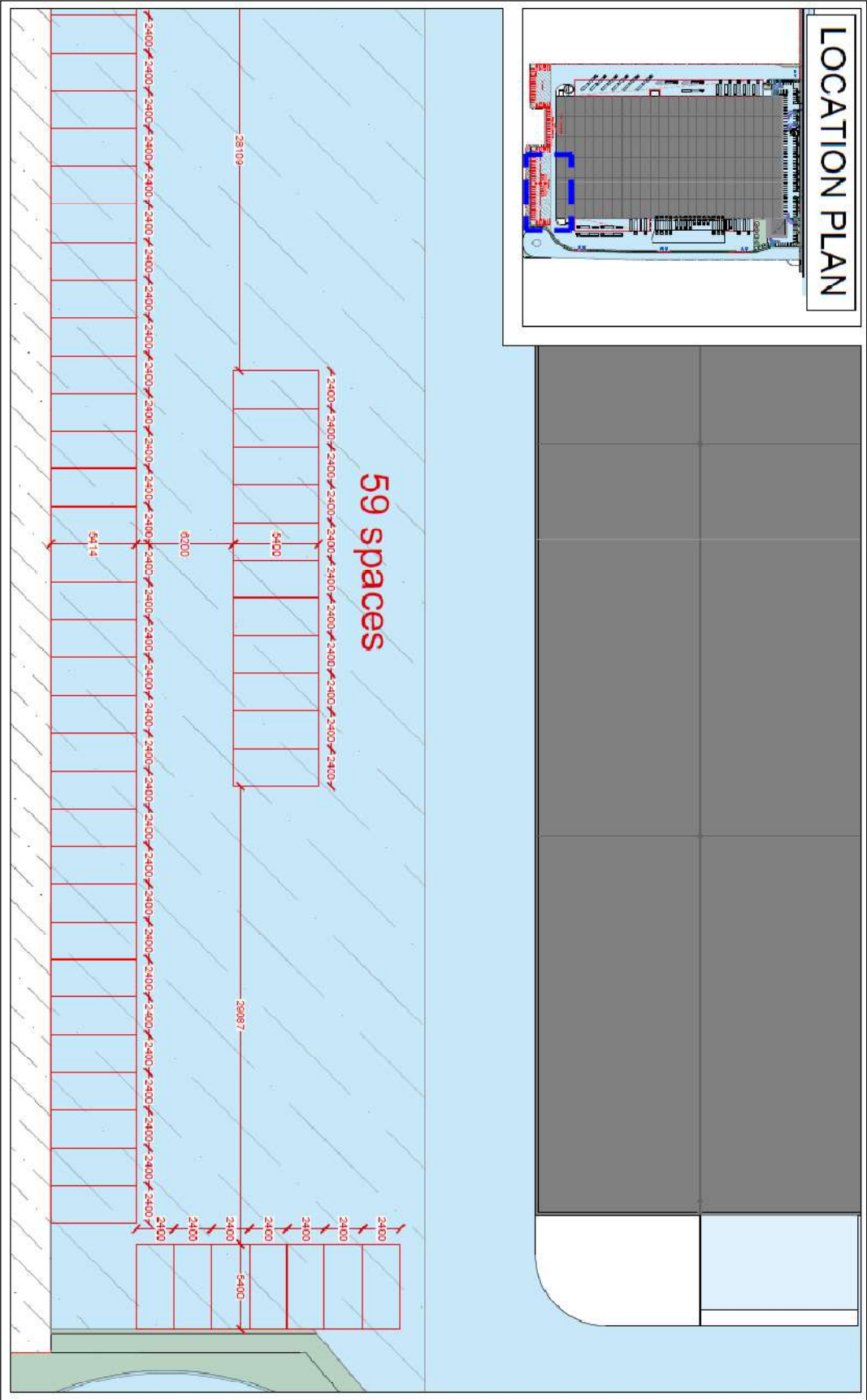
FIGURE 4.15 – PROPOSED OVERFLOW CAR PARKING LAYOUT AND DIMENSIONS
