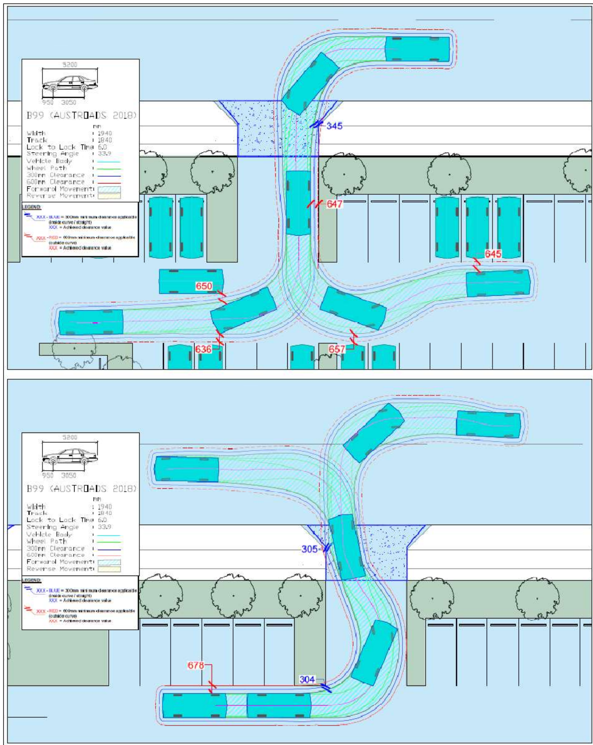
FIGURE 5.5 -SWEPT PATHS FOR B99 DESIGN VEHICLES ENTERING /EXITING THE SITE
