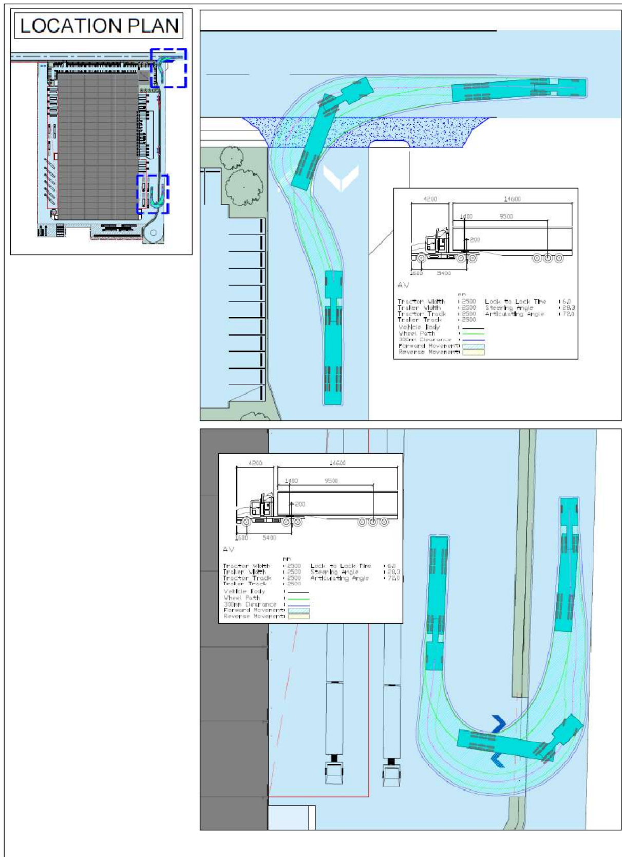
FIGURE 6.2 – VEHICLE SWEEP PATH (ARTICULATED VEHICLE)
