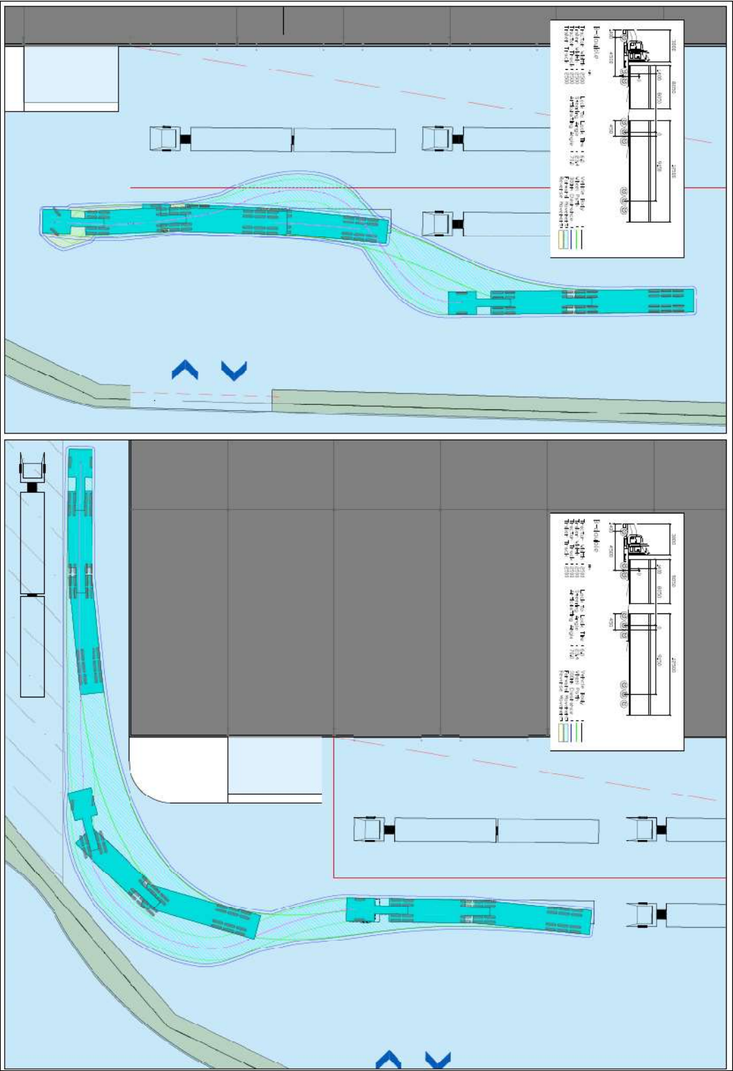
FIGURE 6.10 - VEHICLE SWEEP PATH (B-DOUBLE VEHICLE)
