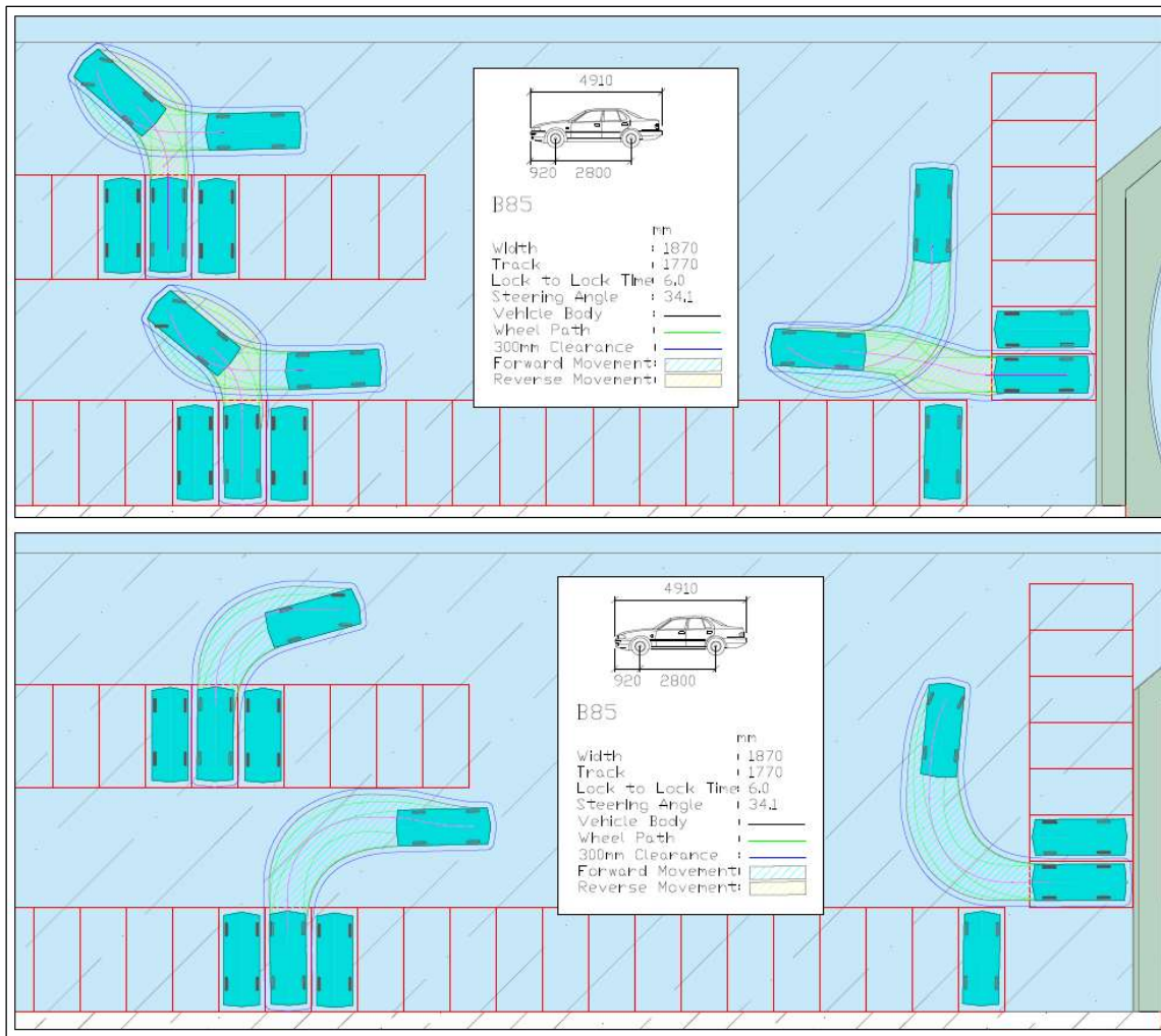
FIGURE 4.16 – SWEEP PATHS FOR A B85 VEHICLE (OVERFLOW CAR PARKING)
