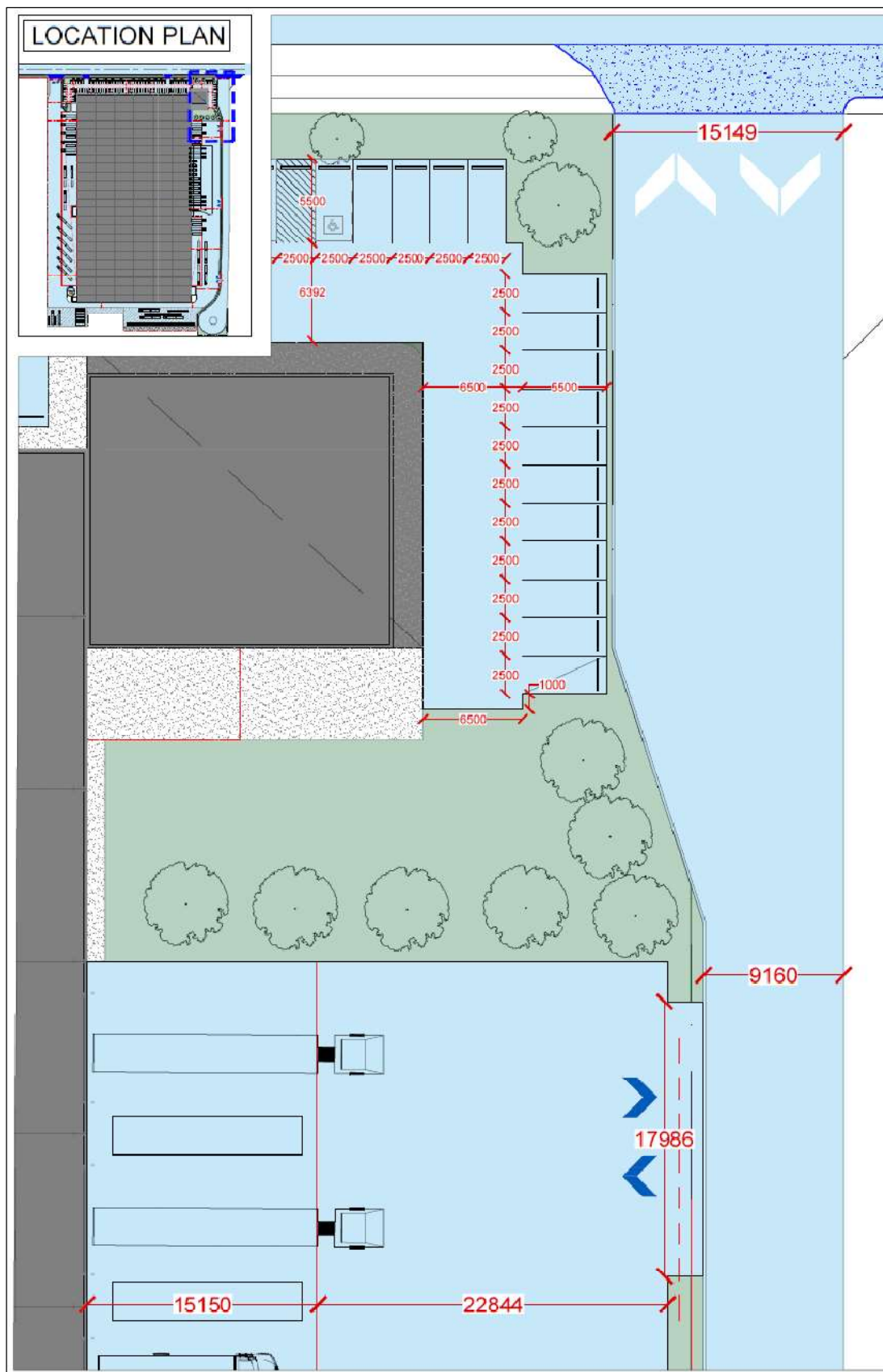
FIGURE 4.5 – PROPOSED CAR PARKING LAYOUT AND DIMENSIONS (EASTERN END)
