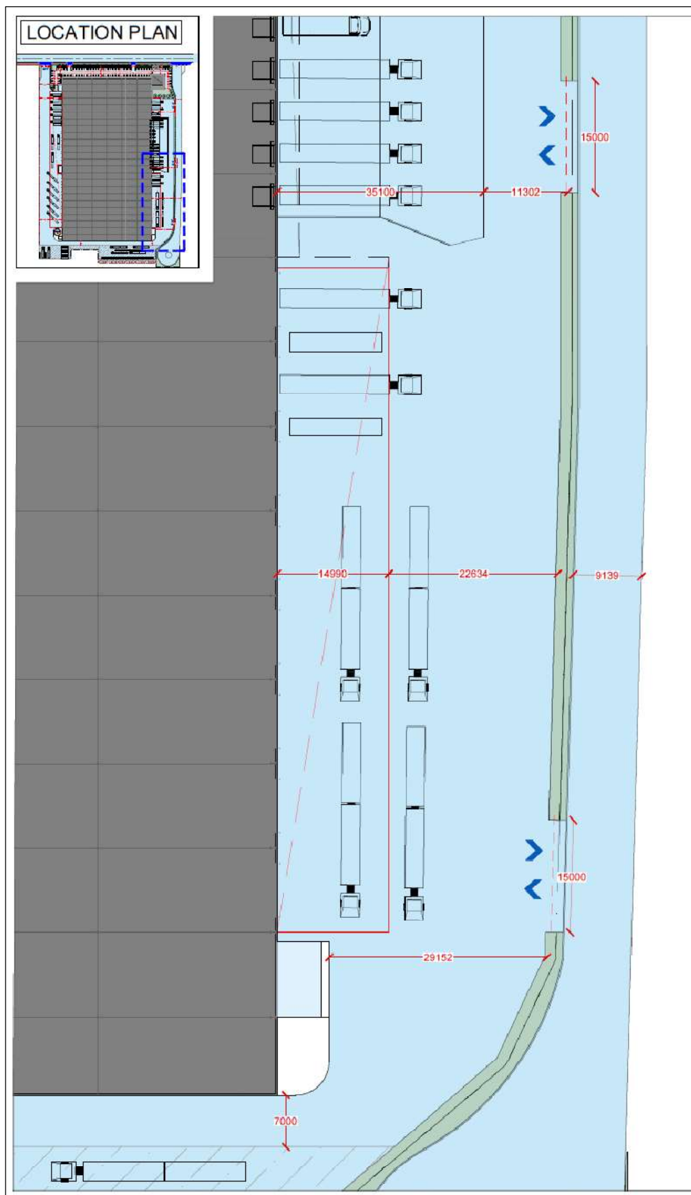
FIGURE 4.6 – PROPOSED CAR PARKING LAYOUT AND DIMENSIONS (EASTERN END)
