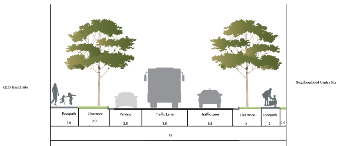
Access Street Section B - Cross-Section
