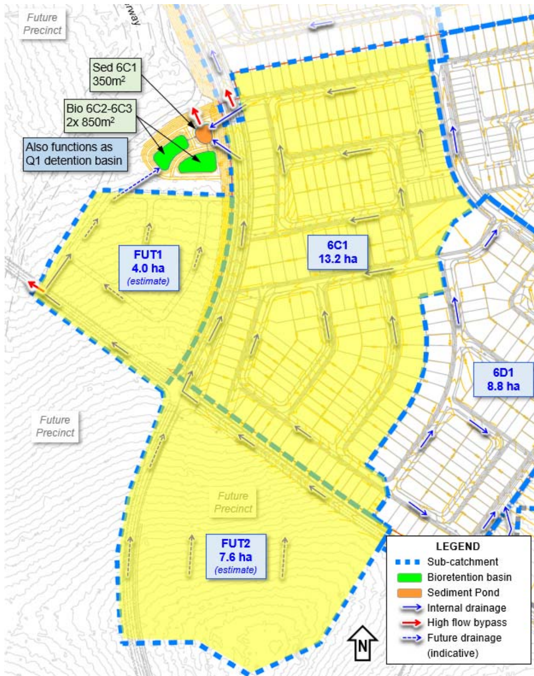
Figure 11: Western catchment layout (extract from Figure 5)
