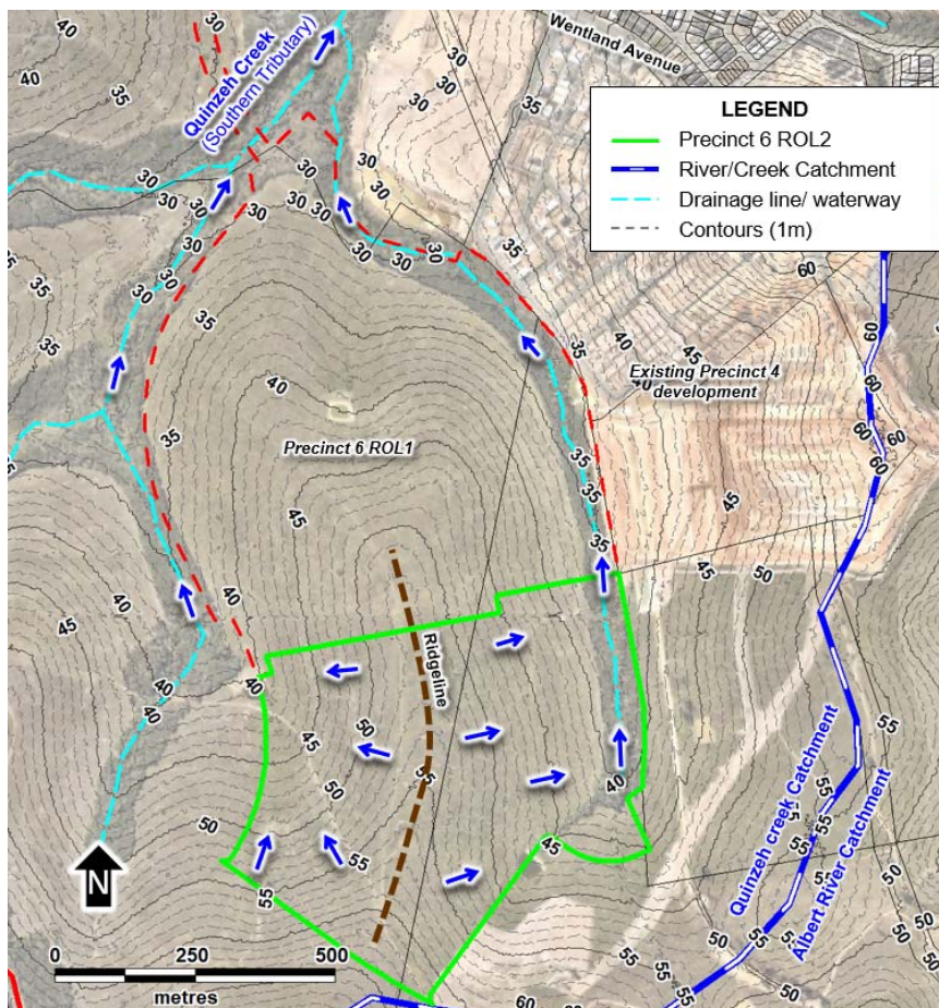
Figure 2: Existing topography, catchments and drainage
