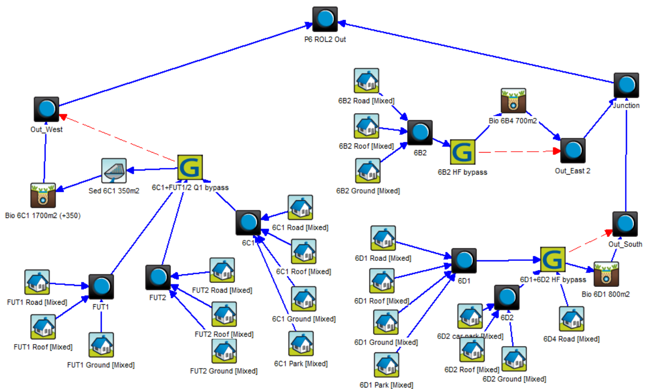
Figure 6: MUSIC model layout
