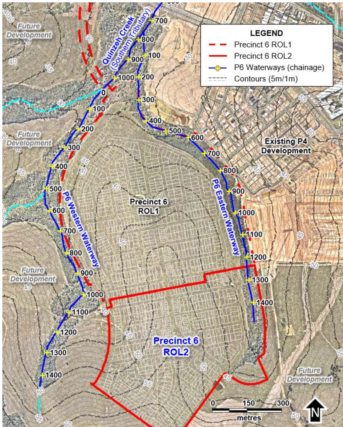
Figure 7: Precinct 6 waterway layout
