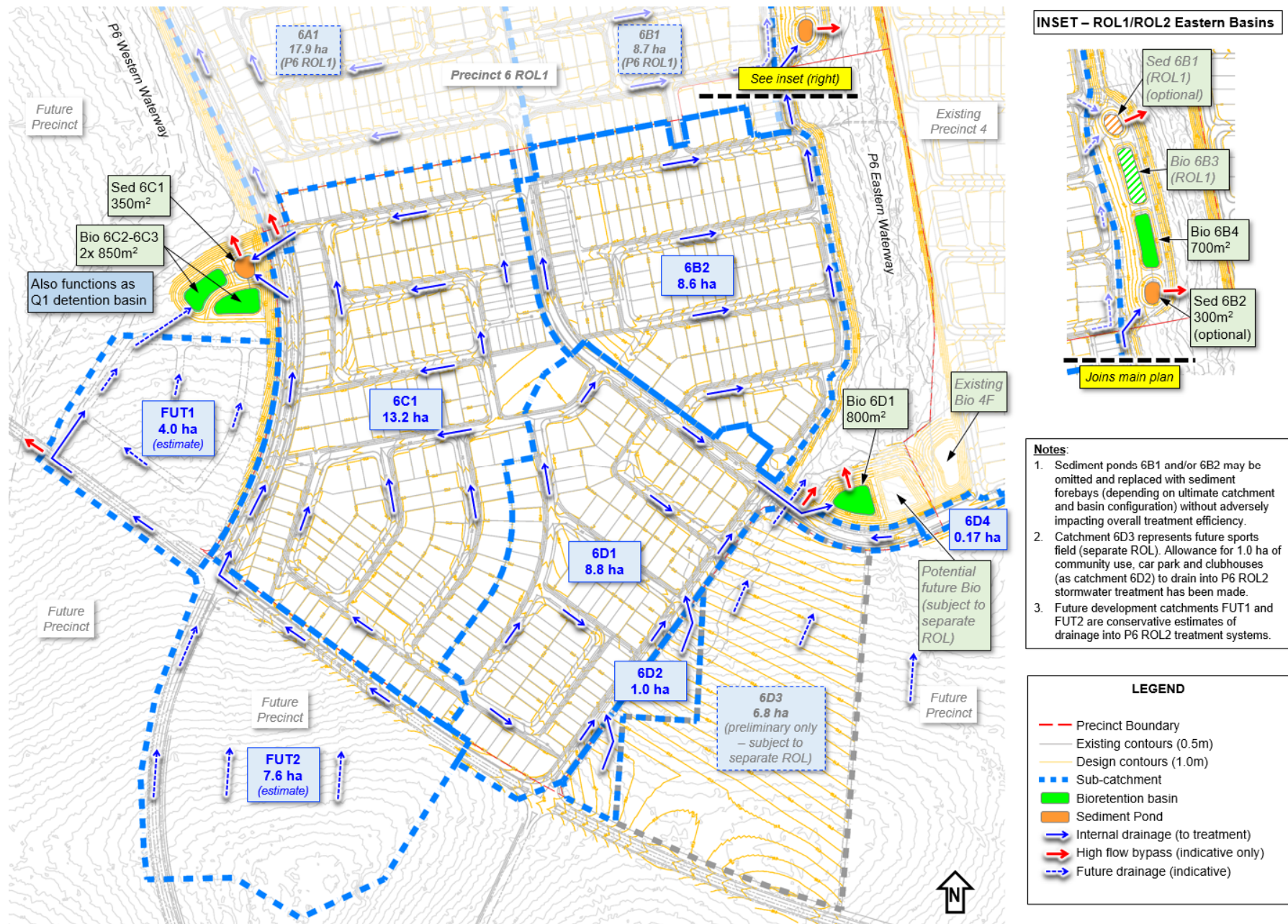
Figure 5: Precinct 6 ROL2 stormwater quality management strategy
