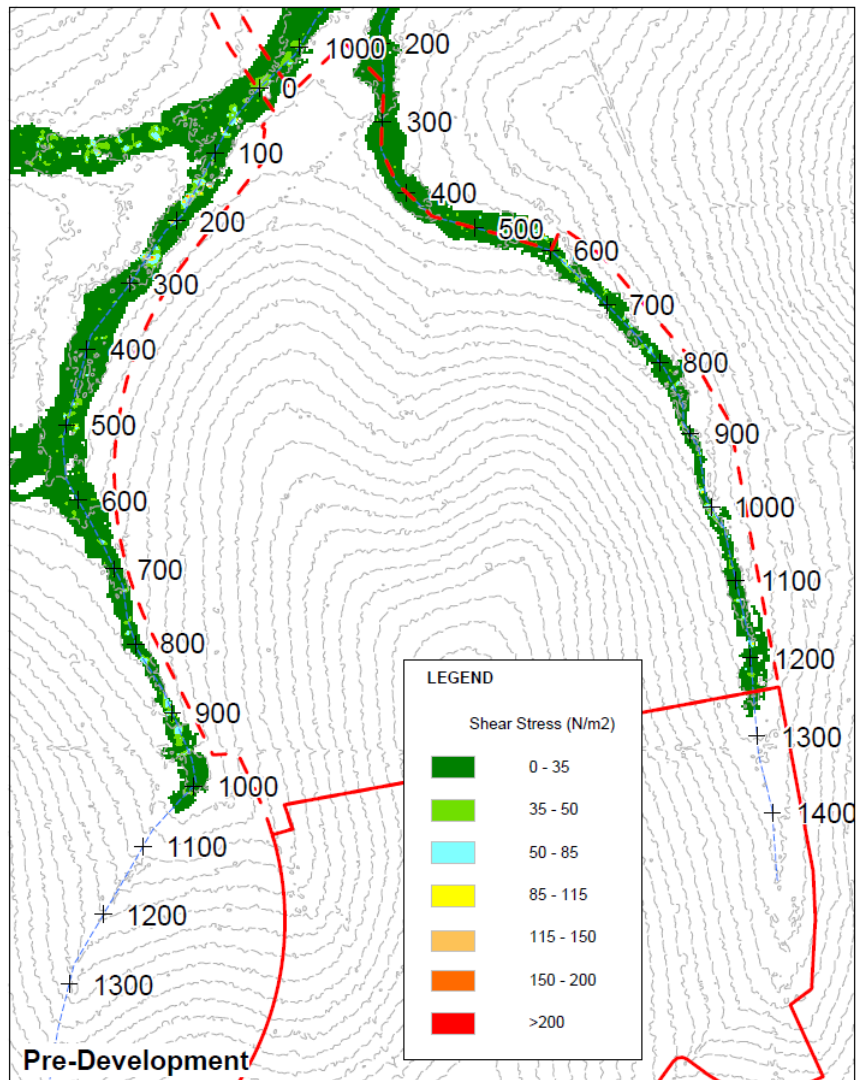
Figure 8: 1 year ARI bed shear stress comparison
