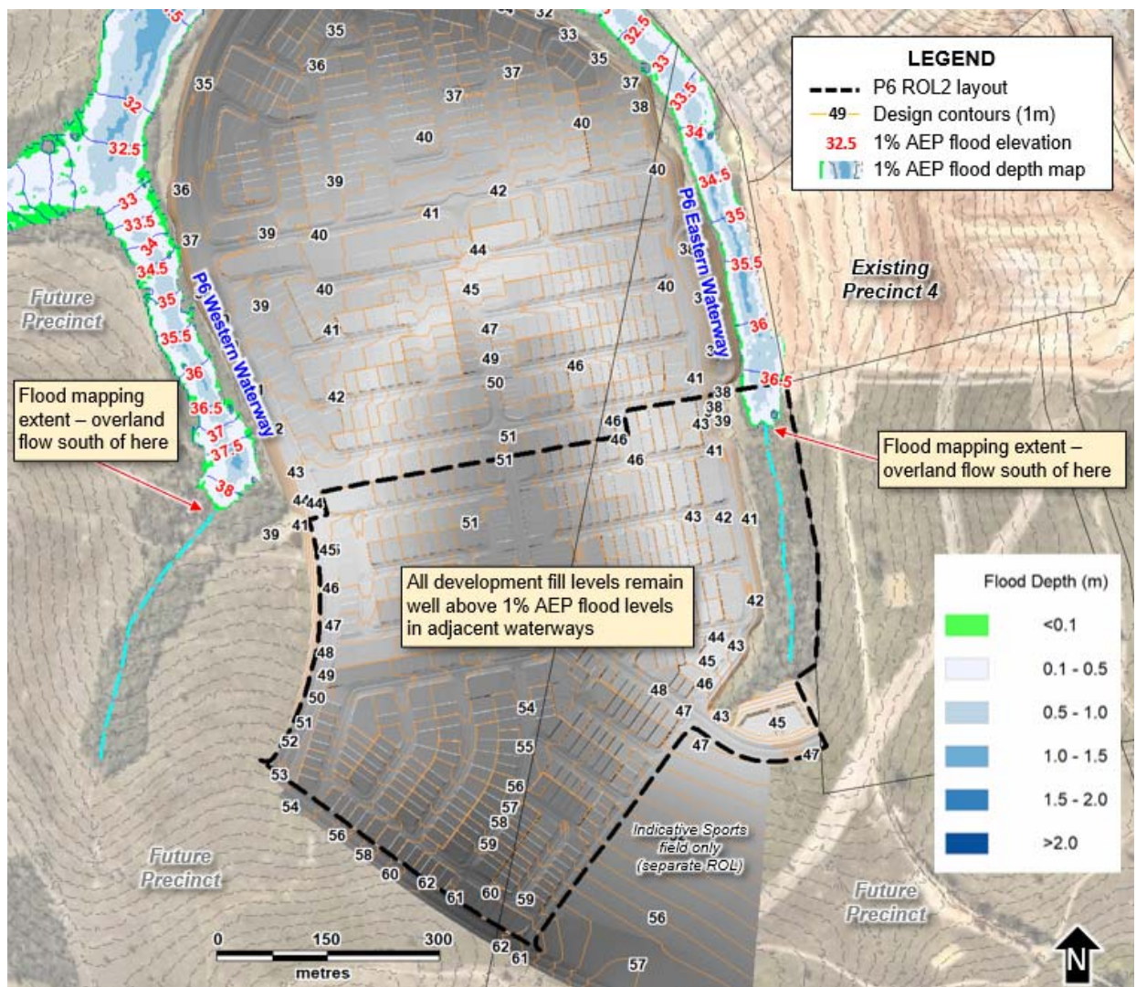
Figure 10: 1% AEP Flood levels and preliminary earthworks
