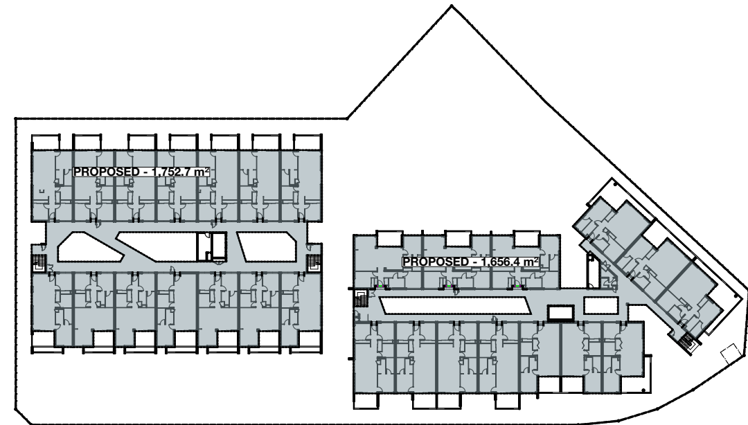
2. LEVEL 2 GFA 1:1000
