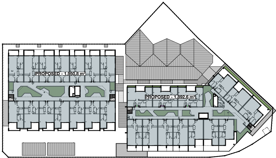
1. LEVEL 1 GFA 1:1000
