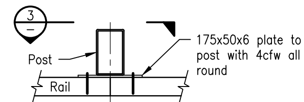
SECTION 2
