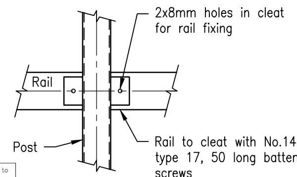
SECTION 3
