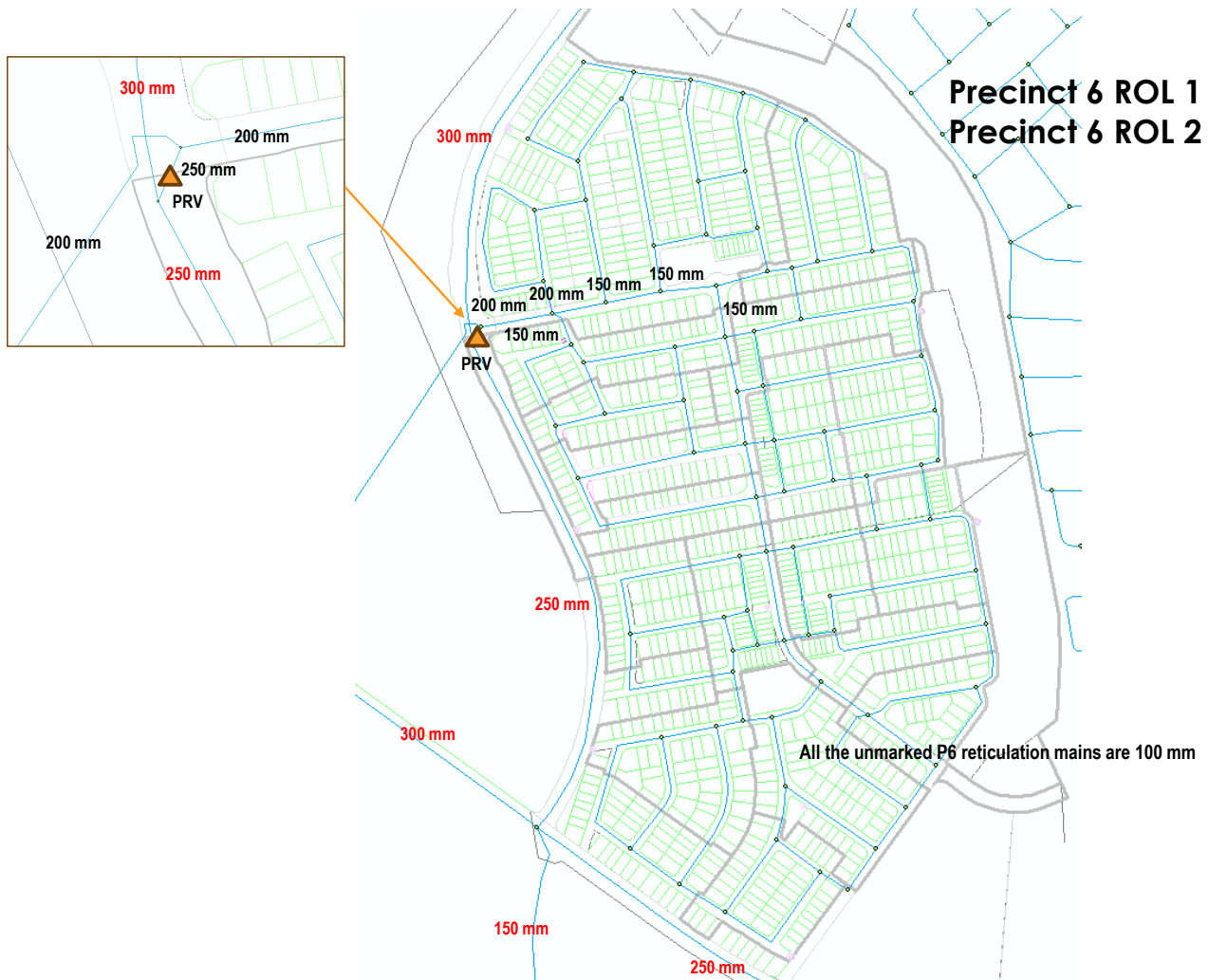
Figure 3: Proposed Precinct 6 ROL 1 Water Reticulation Mains
