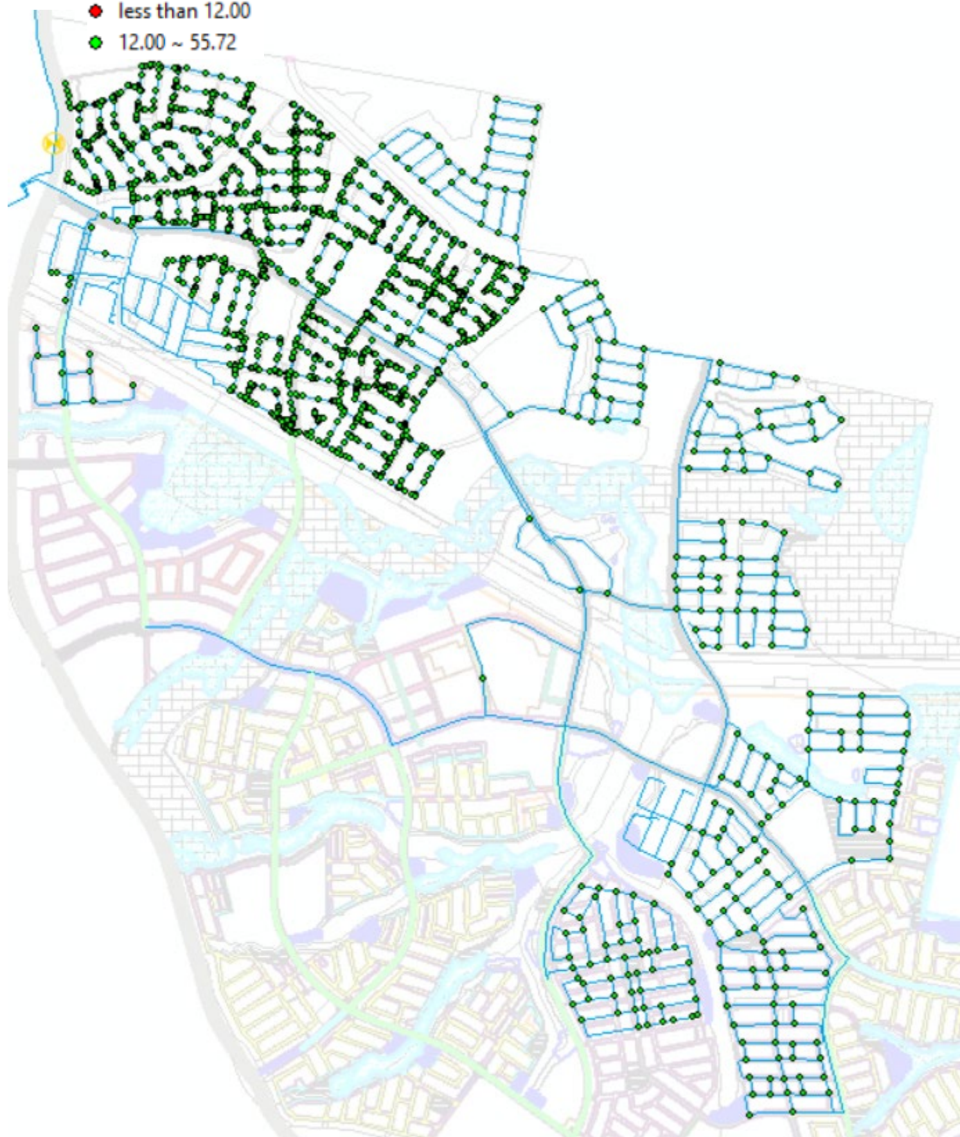
Fire Fighting Residual Pressure (m) (Without Pressure Reduction, LCC operation)
