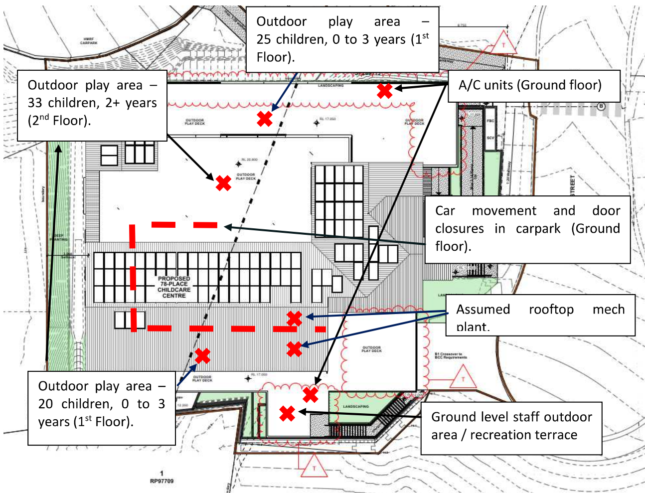
Figure 5 Noise sources considered.
