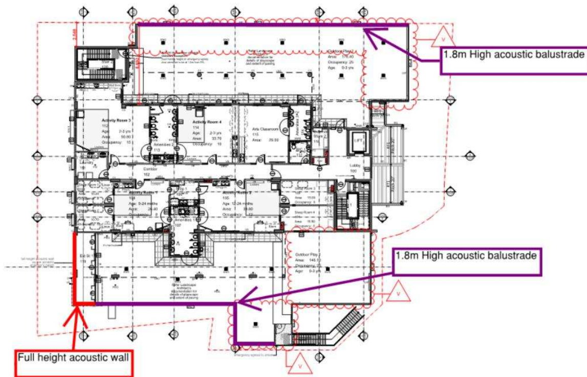
Figure 7 Acoustic treatment locations Level 2
