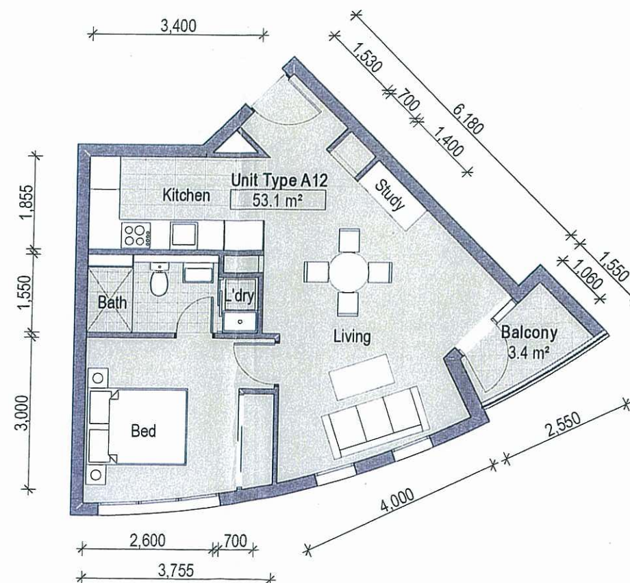
4 Unit A12 SCALE 1:50 @ A1
