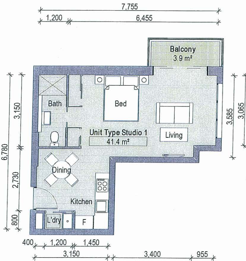
1 Studio 1 SCALE 1:50 @ A1
