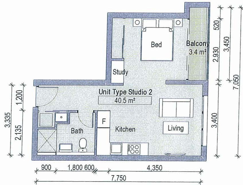
2 Studio 2 SCALE 1:50 @ A1
