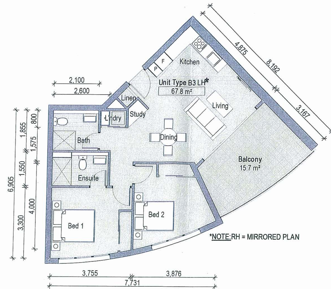
3 Unit B3 SCALE 1:50 @ A1
