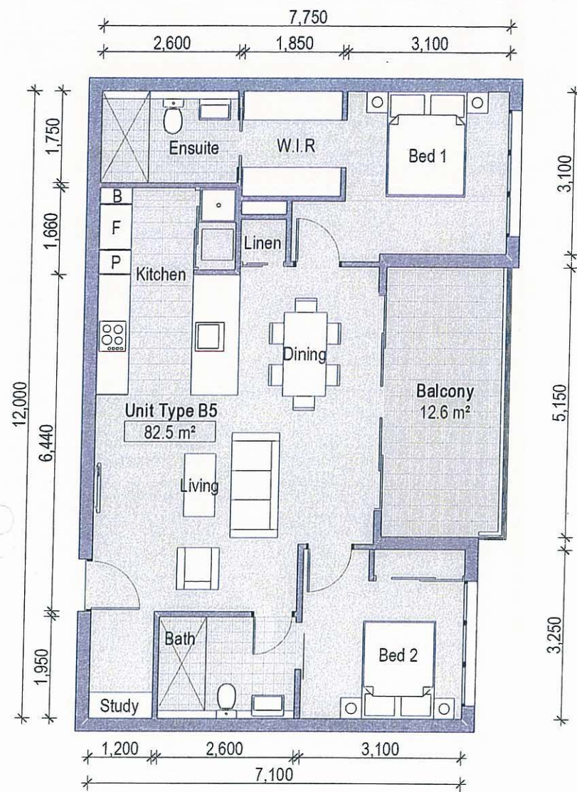
1 Unit B5 SCALE 1:50 @ A1
