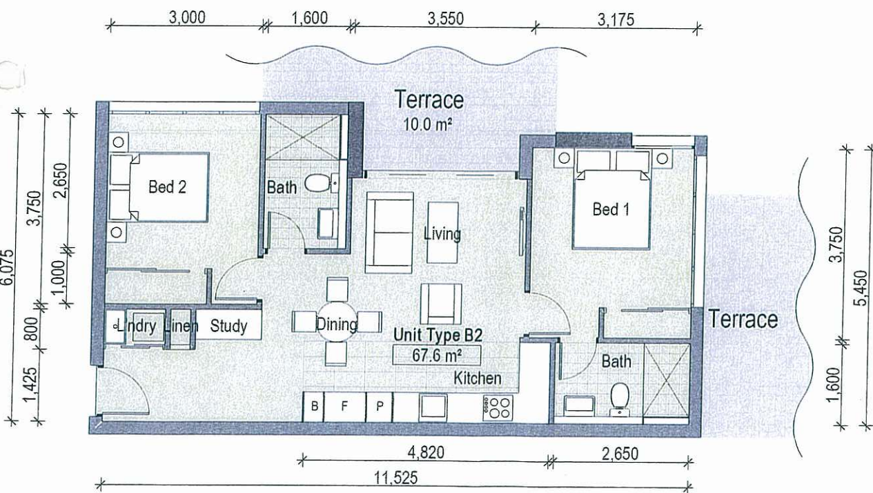
2 Unit B2 - Caretaker's Unit SCALE 1:50 @ A1
