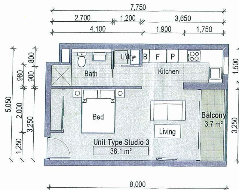
3 Studio 3 SCALE 1:50 @ A1
