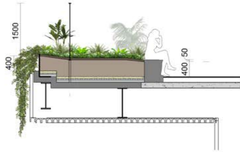
2 Level 1 - Section 2 - 1:50
