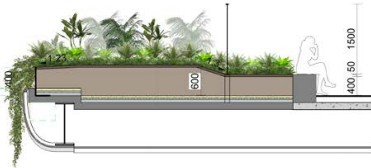
3 Level 1 - Section 3 - 1:50
