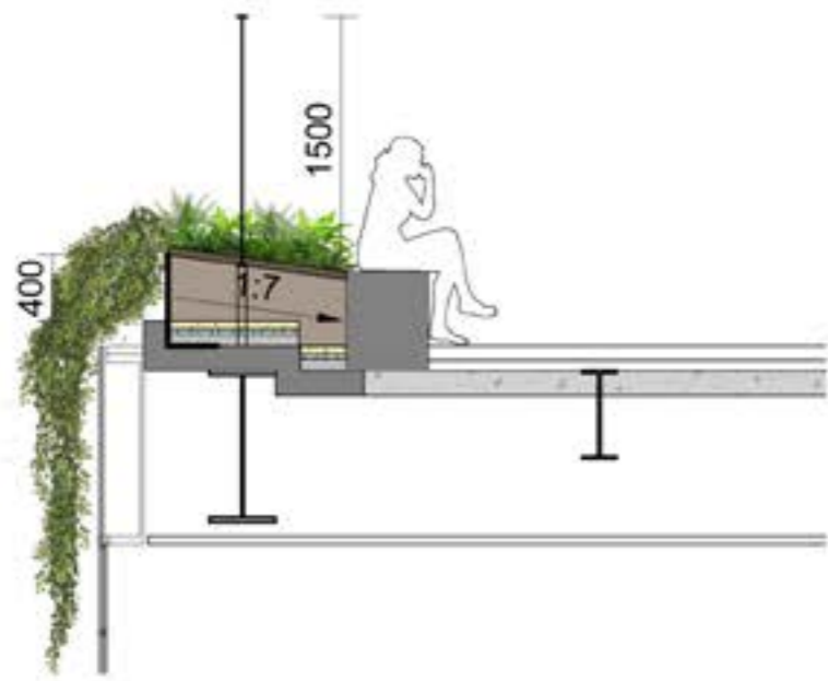
1 Level 3 Section 1 - 1:50
