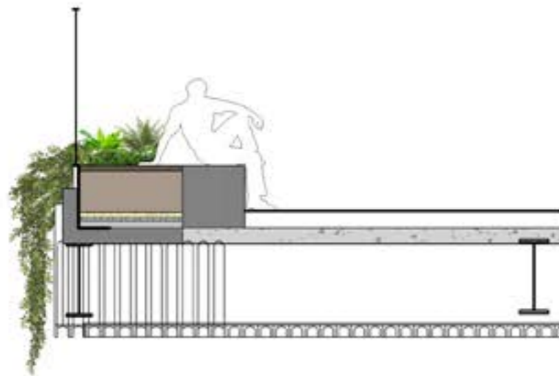
3 Level 2 - Section 3 - 1:50
