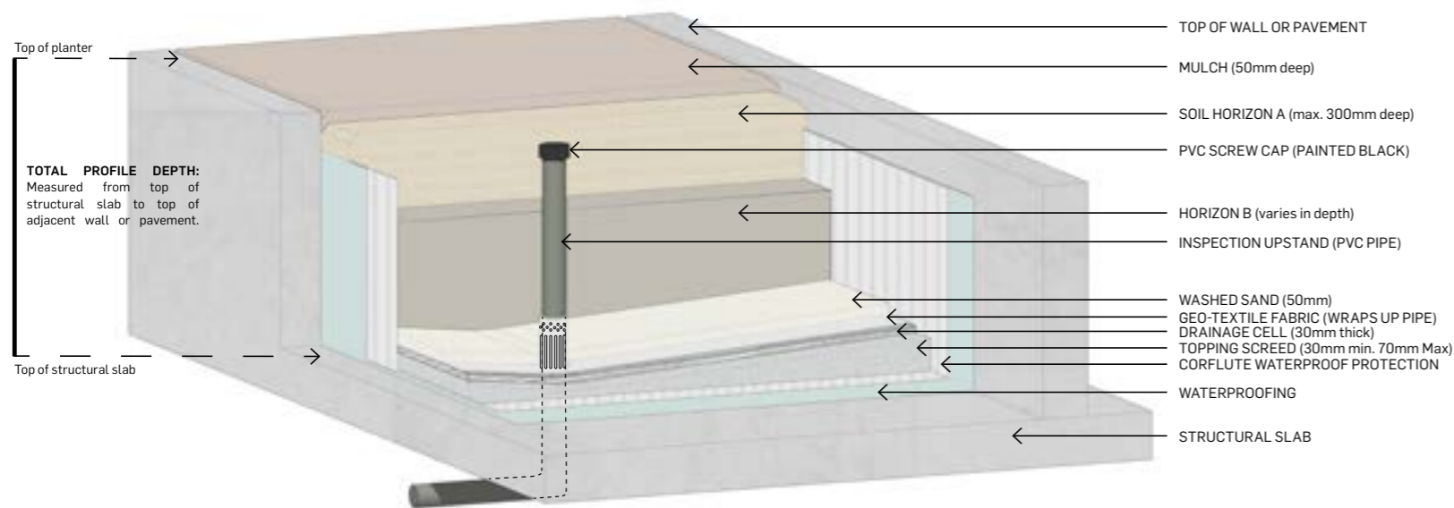
TYPICAL ON-STRUCTURE PLANTER BUILD-UP
