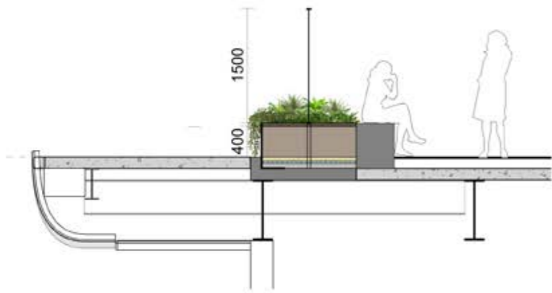
1 Level 1 - Section 1 - 1:50
