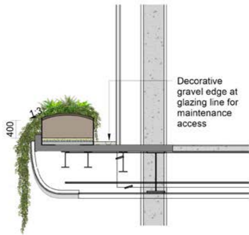
1 Level 2 - Section 1 - 1:50
