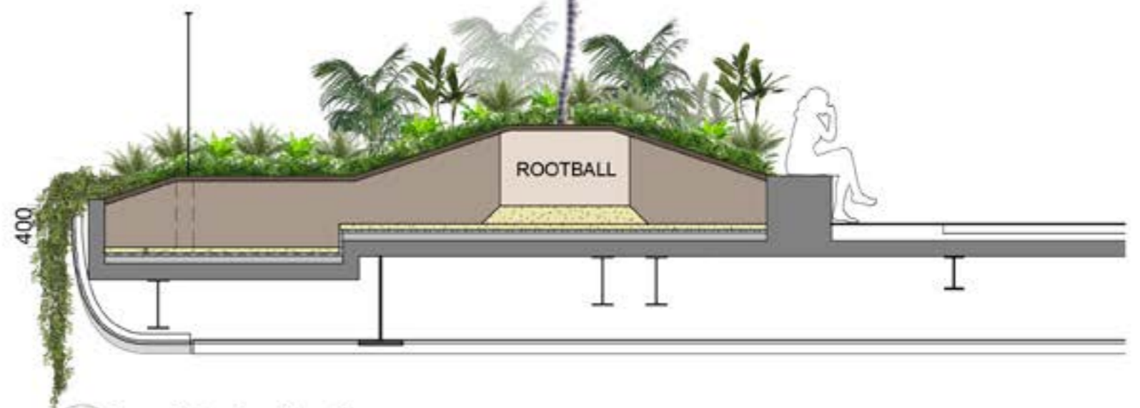
2 Level 2 - Section 2 - 1:50
