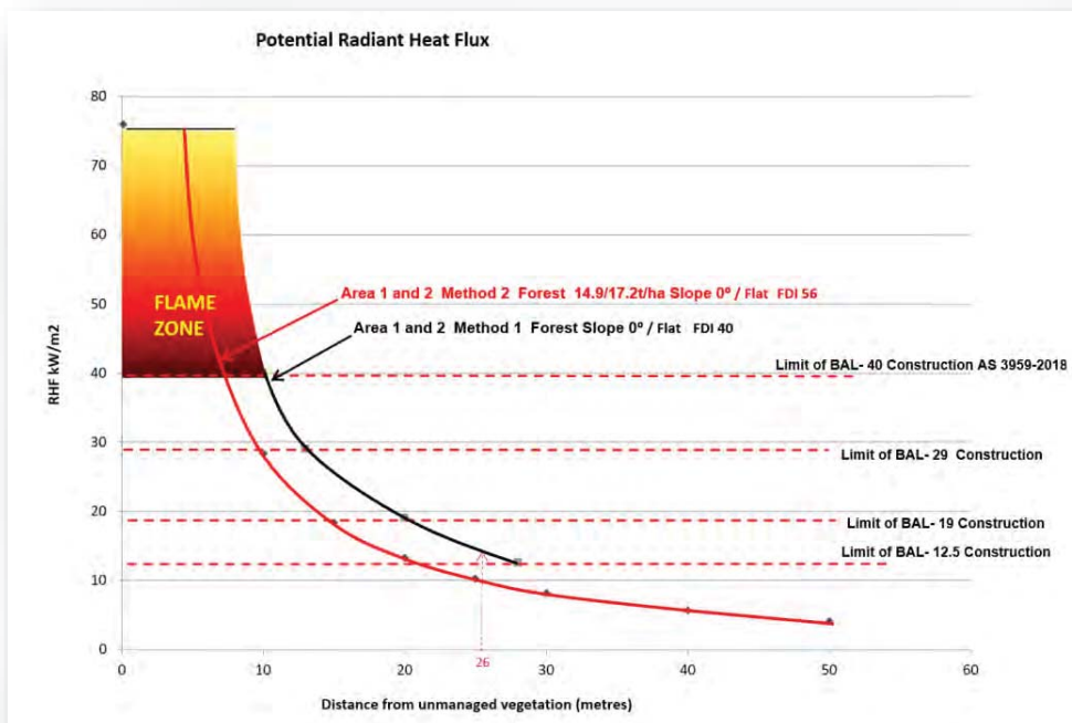
Figure 9. Radiant Heat Flux Predicted by Methods 1 and 2.
