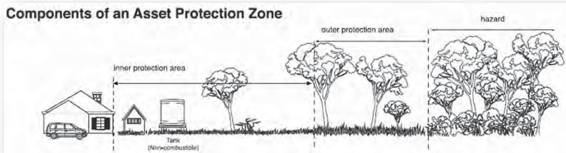
Figure 12. Components of an Asset Protection Zone (APZ)
