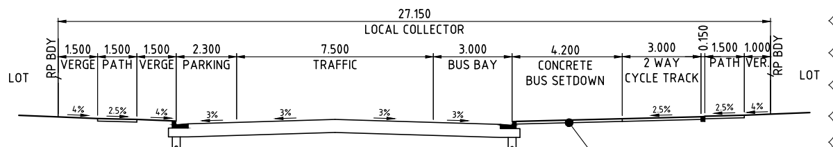
LOCAL COLLECTOR - FUTURE SCHOOL FRONTAGE
