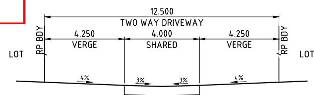
TWO WAY DRIVEWAY
