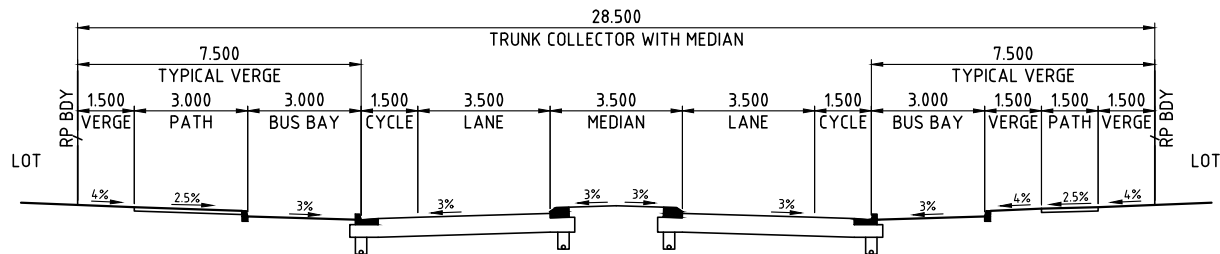
TRUNK COLLECTOR WITH MEDIAN (WITH BUS BAY)
