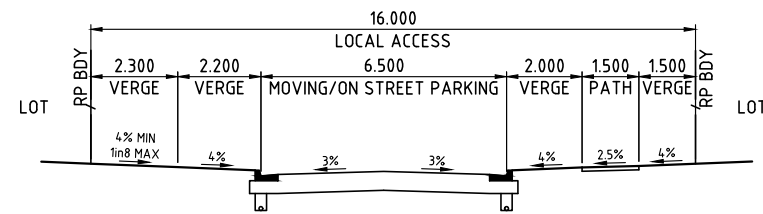
LOCAL ACCESS STREET
