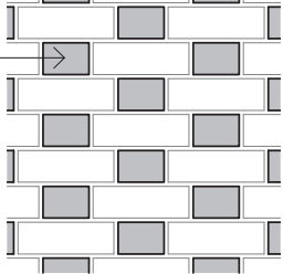
5 BRICK RECESS DETAIL 30.01 Scale at A1: 1 : 10
