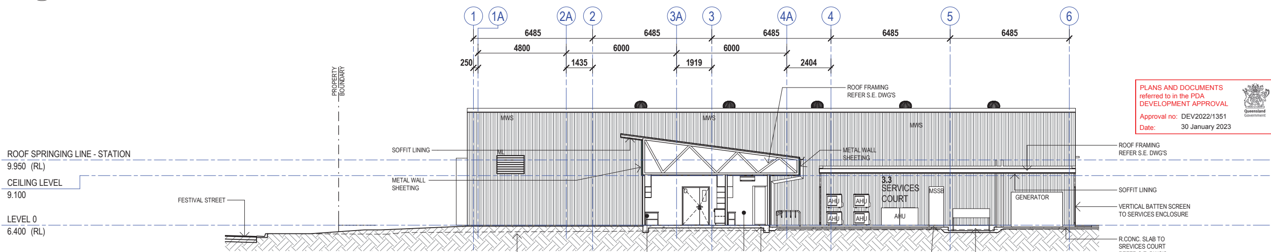
4 SECTION 4 20.01 Scale at A1: 1 : 100
