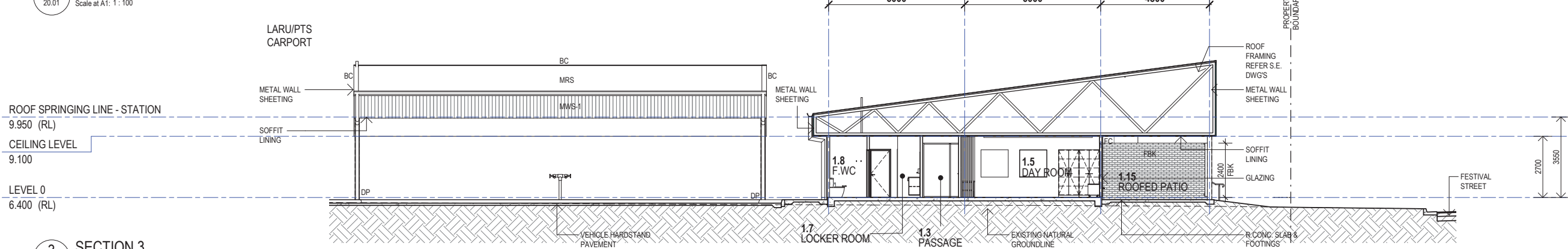
3 SECTION 3 20.01 Scale at A1: 1 : 100
