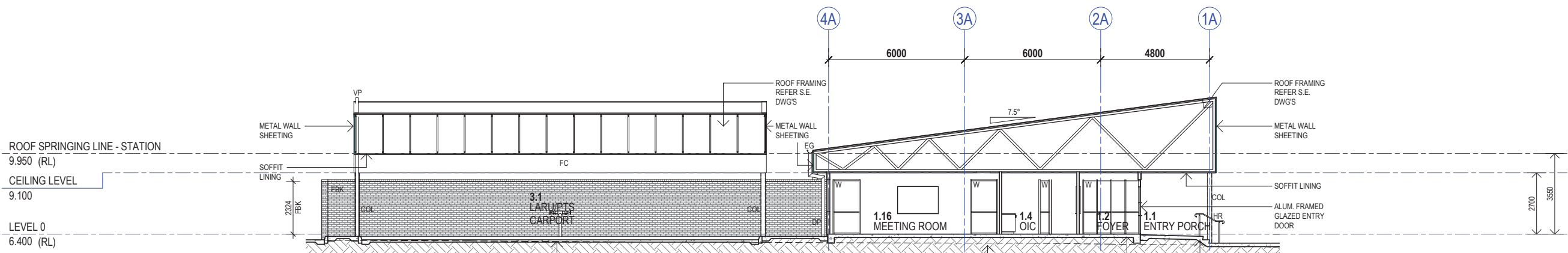
1 SECTION 1 20.01 Scale at A1: 1 : 100
