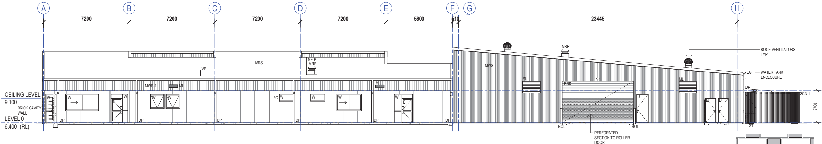
3 SOUTH ELEVATION 23.01 Scale at A1: 1 : 100
