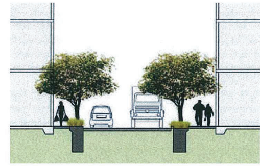
SHORT STREET - SECTION A-A
