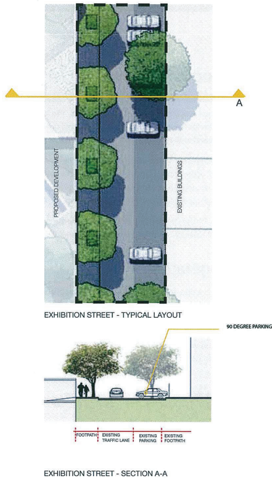
Figure 22 – Indicative Exhibition Street Section
