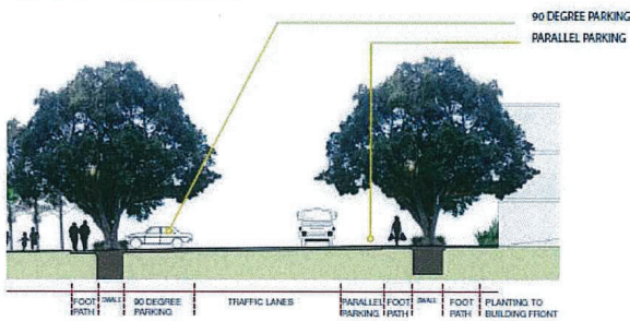
SUTTON ST - SECTION A-A
