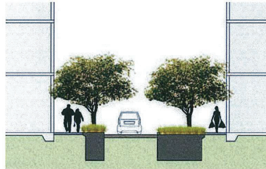
LITTLE WATER STREET - TYPICAL LAYOUT
