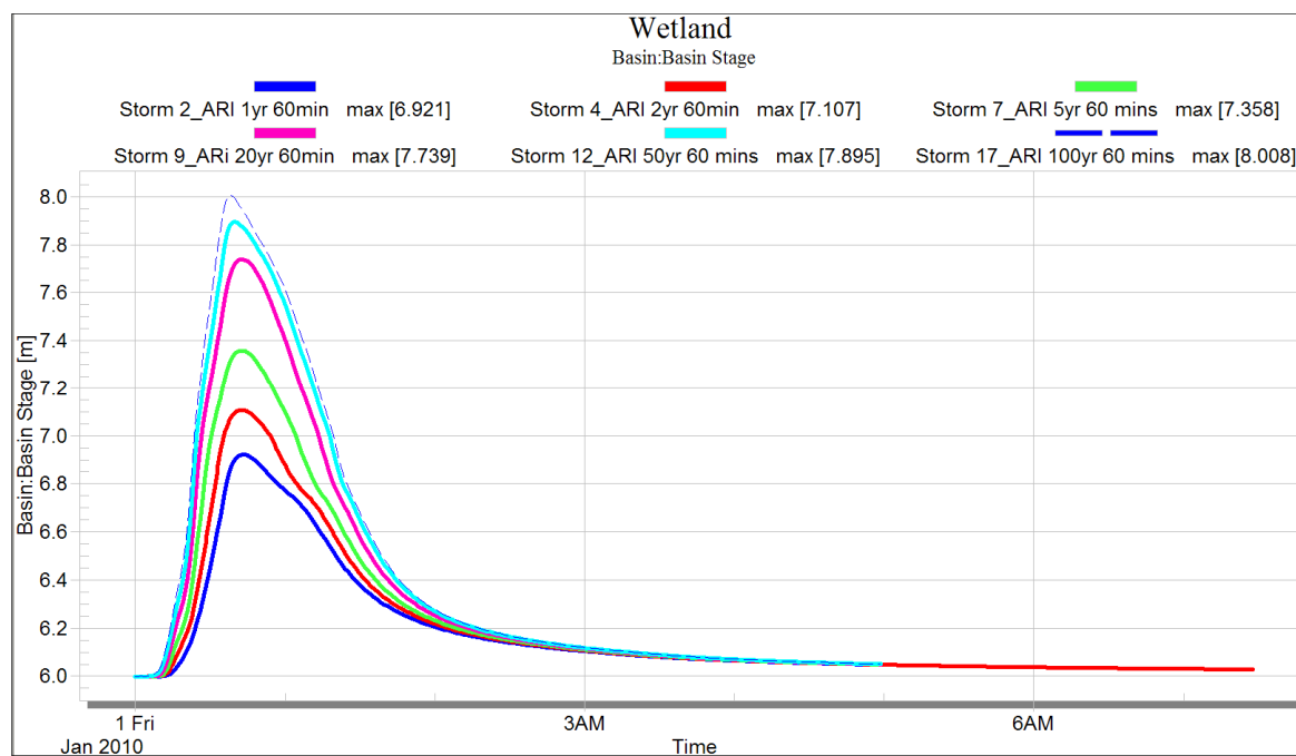
Figure 4.1 Stage Hydrograph in the proposed wetland
