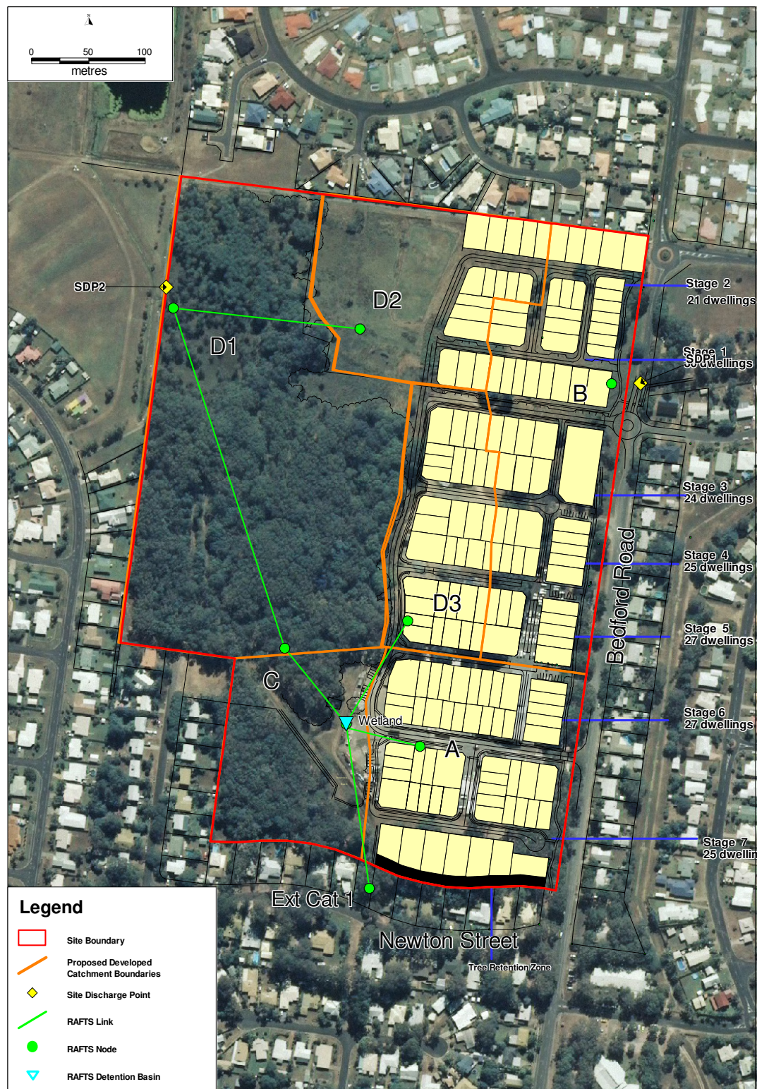
Figure 3.1 Proposed RAFTS Model Configuration
