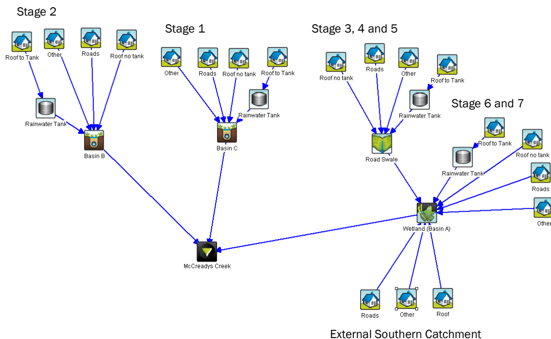
Figure 7.1 MUSIC Model Configuration
