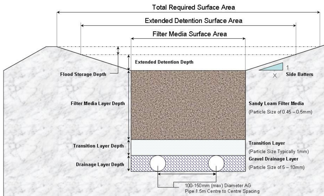
Figure 6.1 Typical Cross Section of a Bio-filtration system
