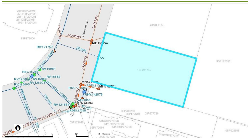
Figure 1: Existing infrastructure within the vicinity of the subject site
