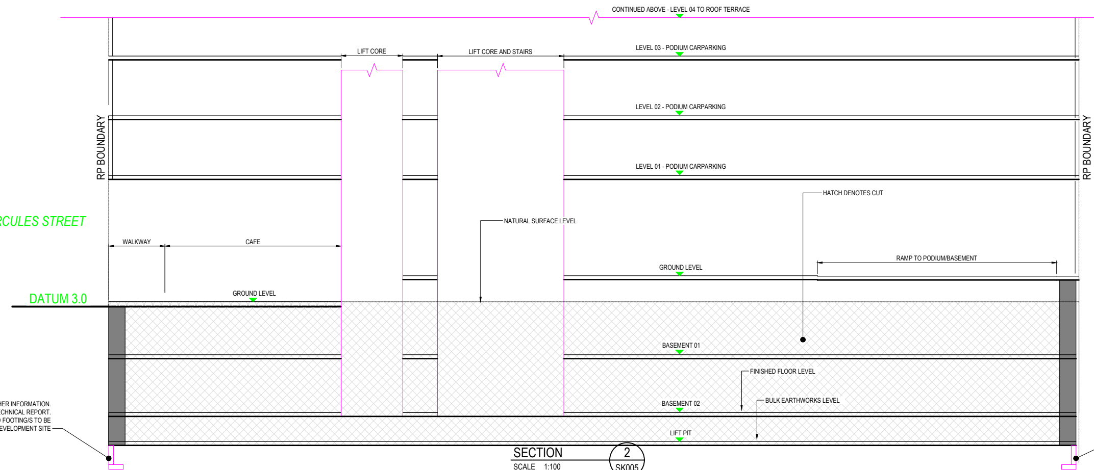
SECTION 1 SCALE 1:100 SK005
