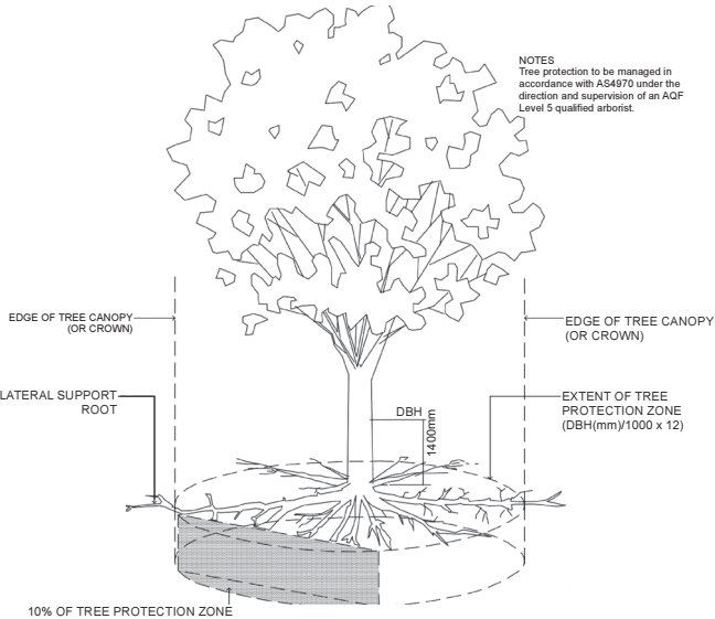
Tree Protection Zone - Detail (not to scale)
