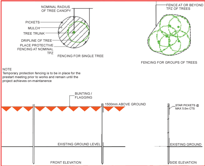
Tree Protection Fencing - Detail (not to scale)
