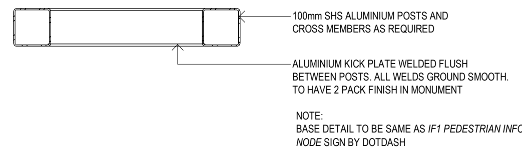
7 EXTERNAL PILLAR SIGN - PLAN DETAIL 1 1 : 10
