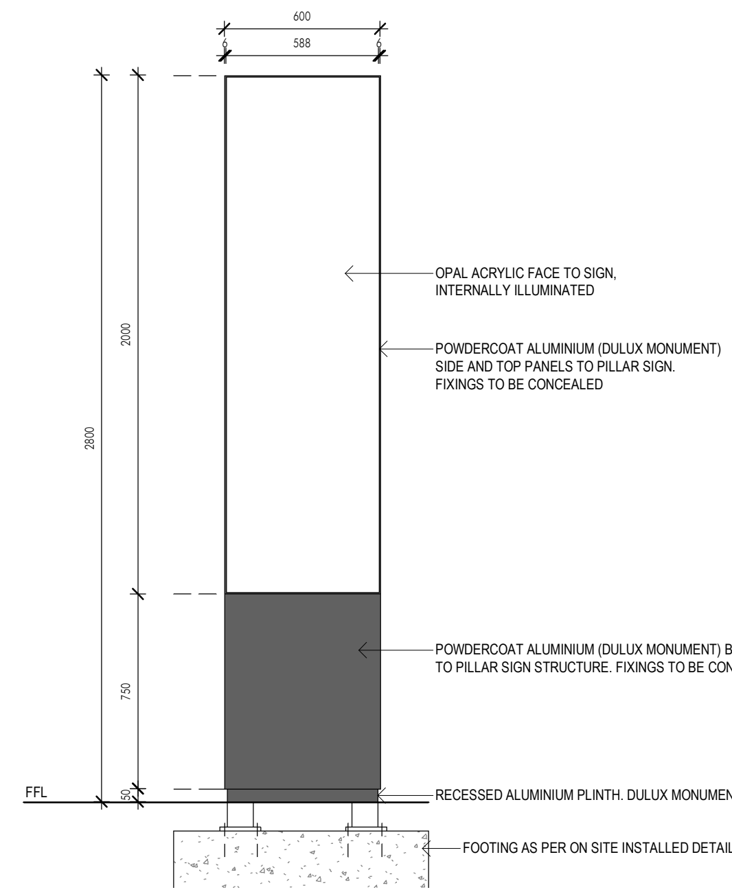
5 EXTERNAL PILLAR SIGN - REAR ELEVATION 1 : 20
