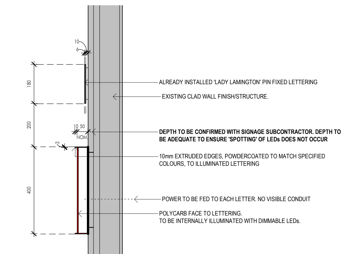
3 ENTRY - ILLUMINATED LETTING SECTION DETAIL 1 : 10
