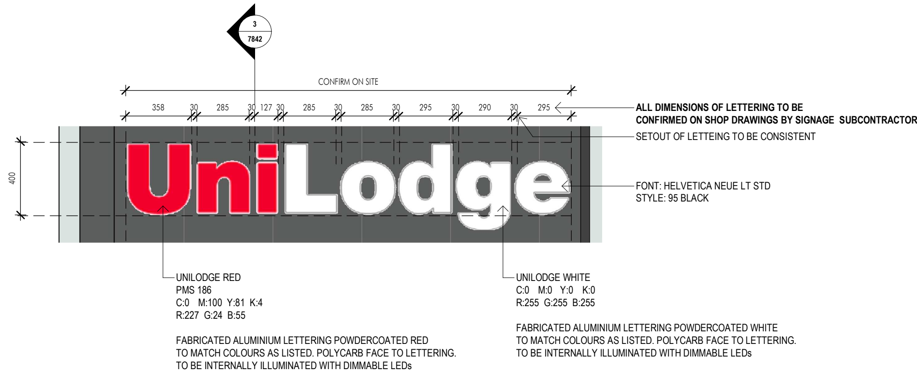
2 ENTRY - EXTERNAL UNILODGE SIGNAGE 1 : 20
