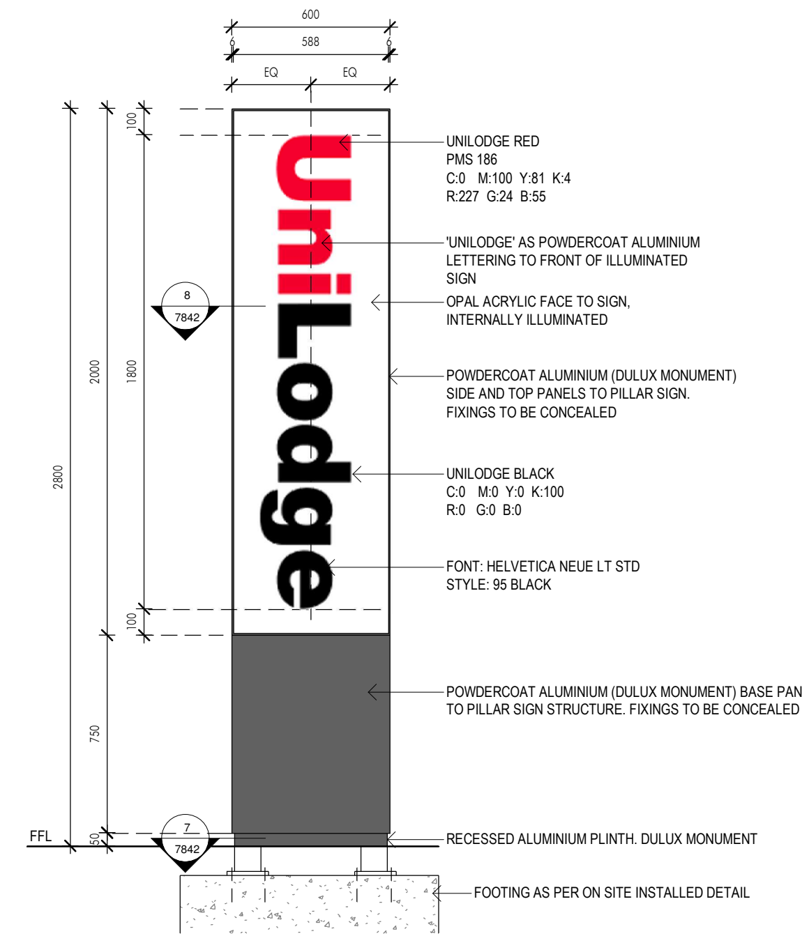
4 EXTERNAL PILLAR SIGN - FRONT ELEVATION 1 : 20
