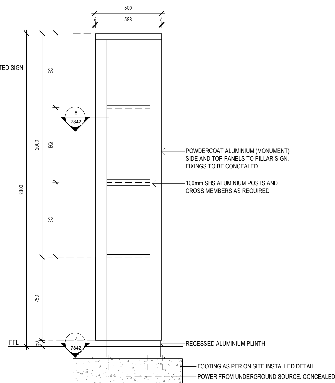
9 EXTERNAL PILLAR SIGN - ELEVATION SECTION 1 : 20
