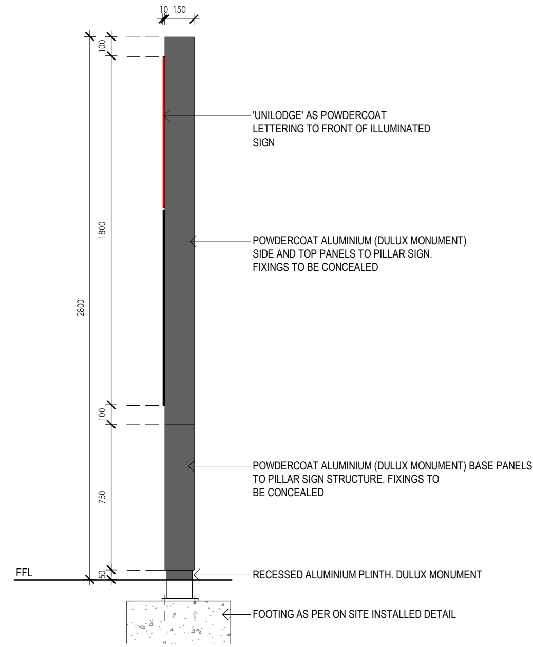
6 EXTERNAL PILLAR SIGN - SIDE ELEVATION 1 : 20
