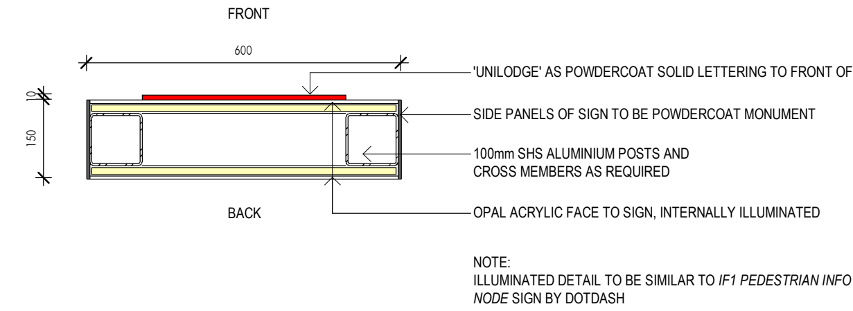
8 EXTERNAL PILLAR SIGN - PLAN DETAIL 2 1 : 10
