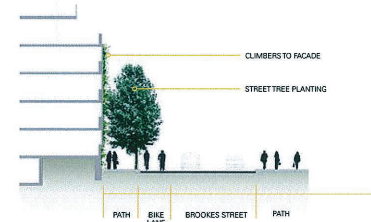
BROOKES STREET - TYPICAL SECTION
