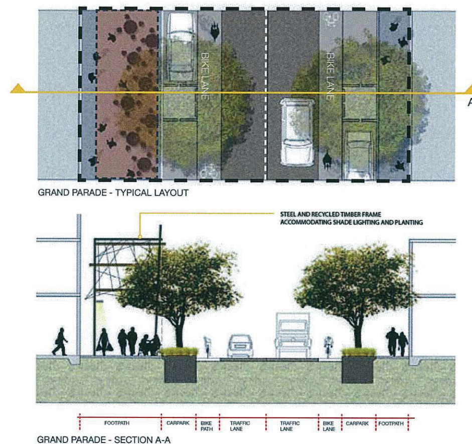
Figure 13 – Indicative Grand Parade Section
