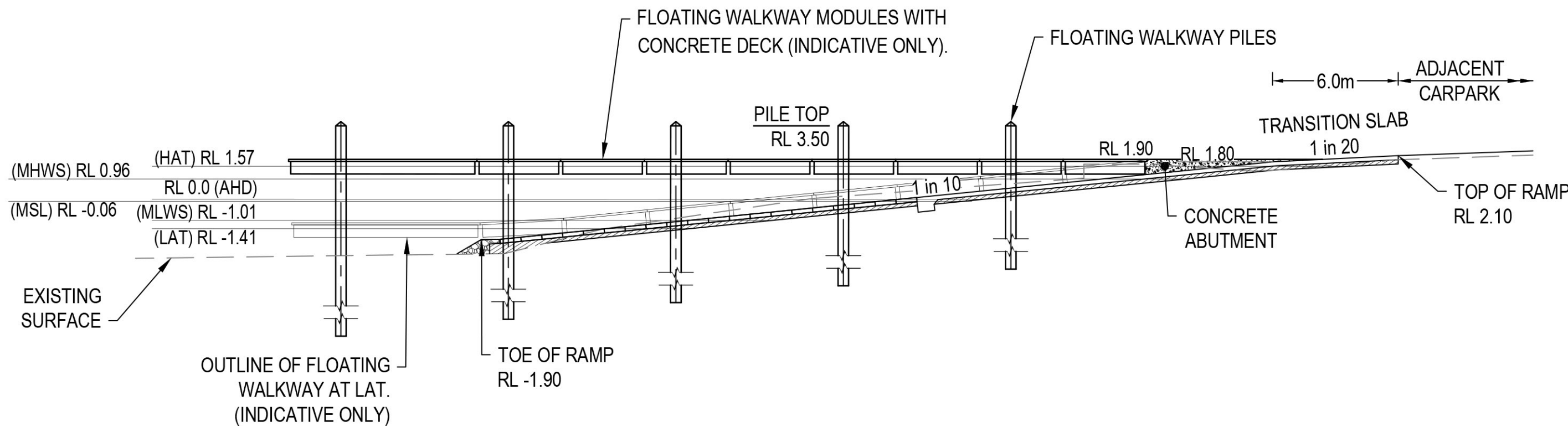
SECTION A SCALE 1:200
