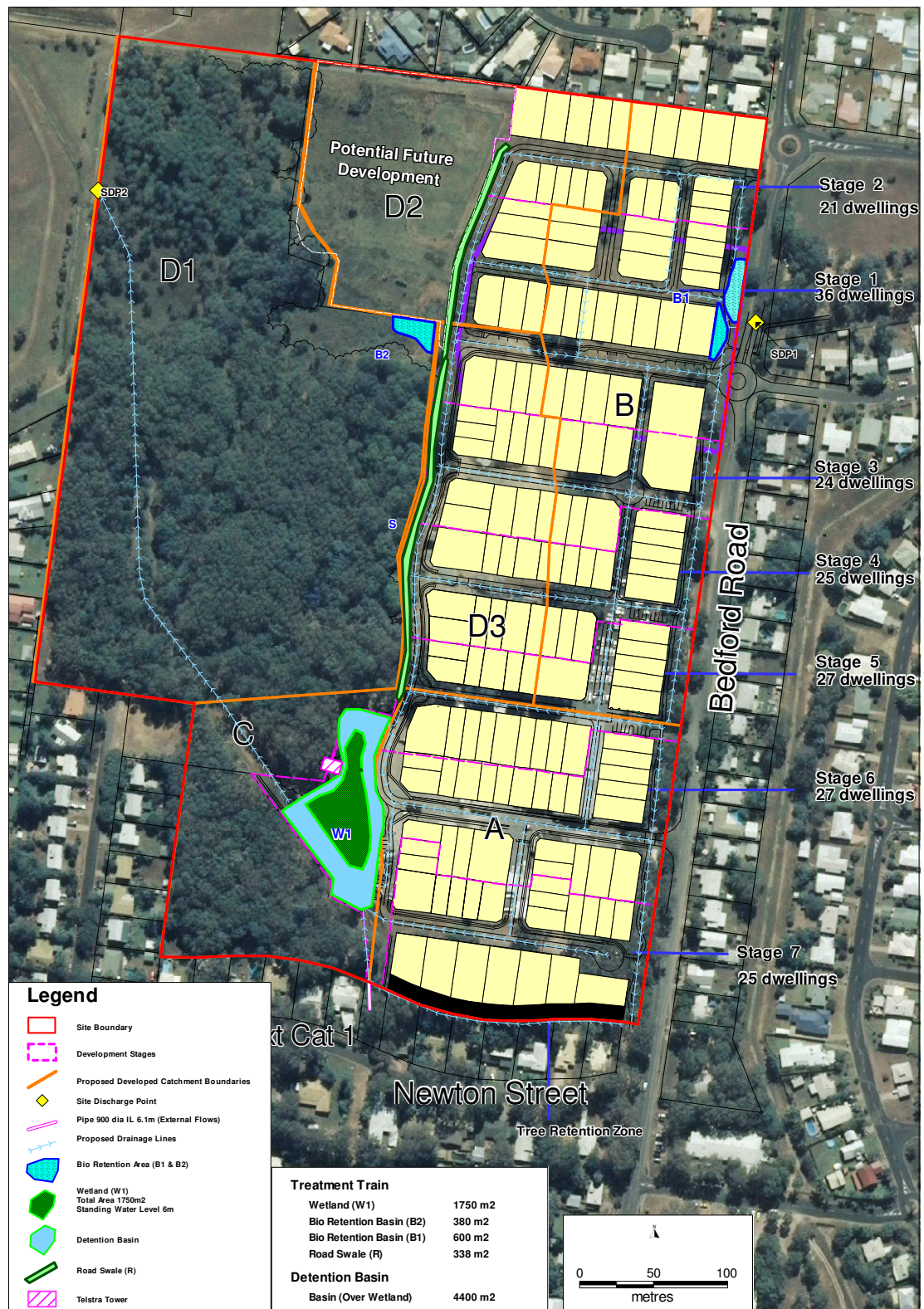
Figure 2.3 Proposed Developed Conditions and Stormwater Management Measures
