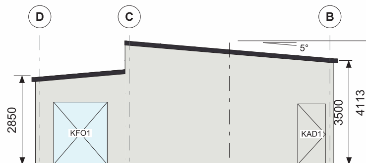
ELEVATION GRID 4
