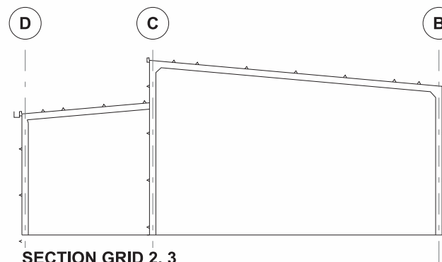
SECTION GRID 2, 3
