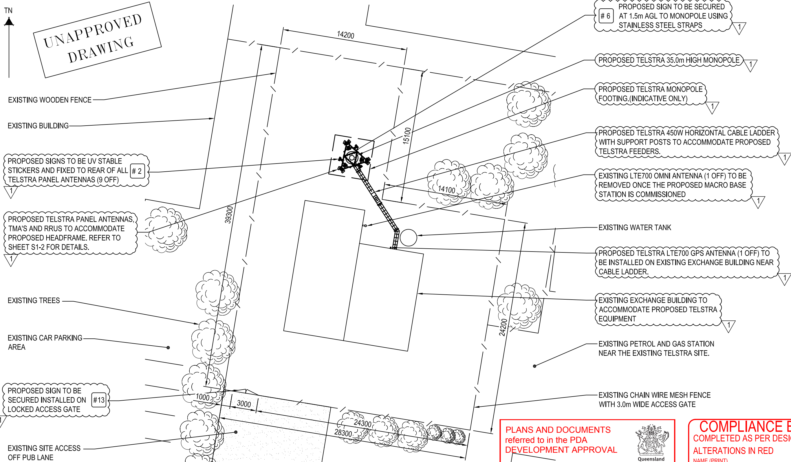
SITE LAYOUT SCALE 1:250 5m 0 5m 10m SCALE 1:250
