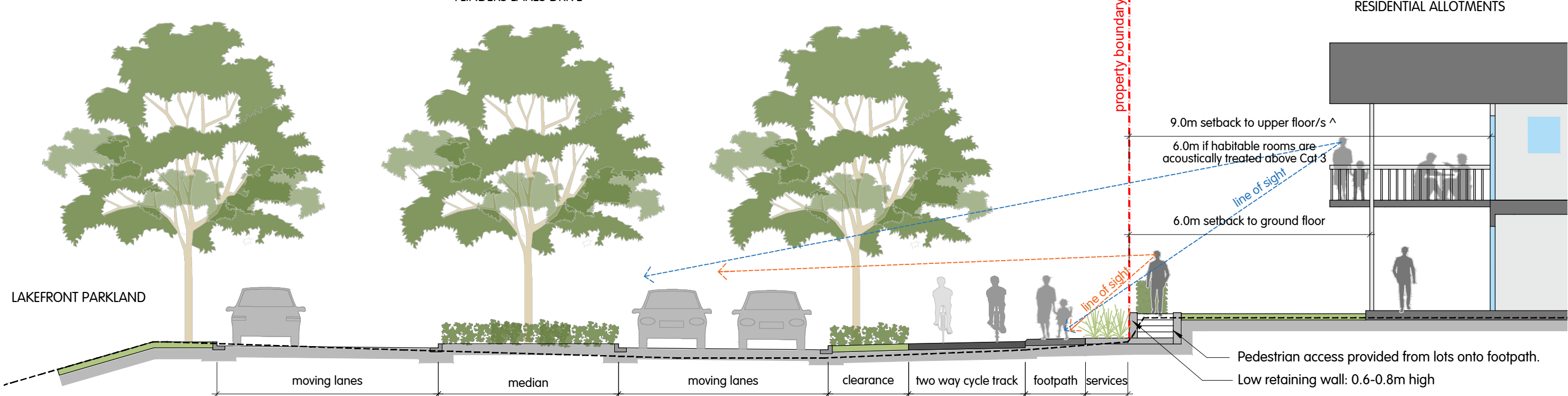
Typical Cross-section OPTION 2 - NO ACOUSTIC FENCE
