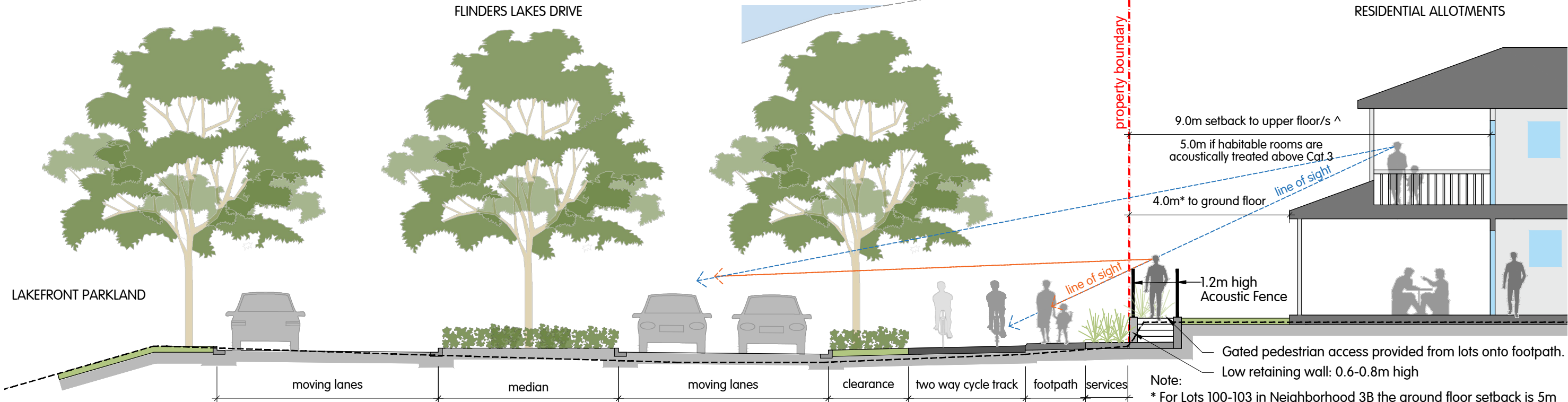
Typical Cross-section OPTION 1 - 1.2M HIGH ACOUSTIC FENCE
