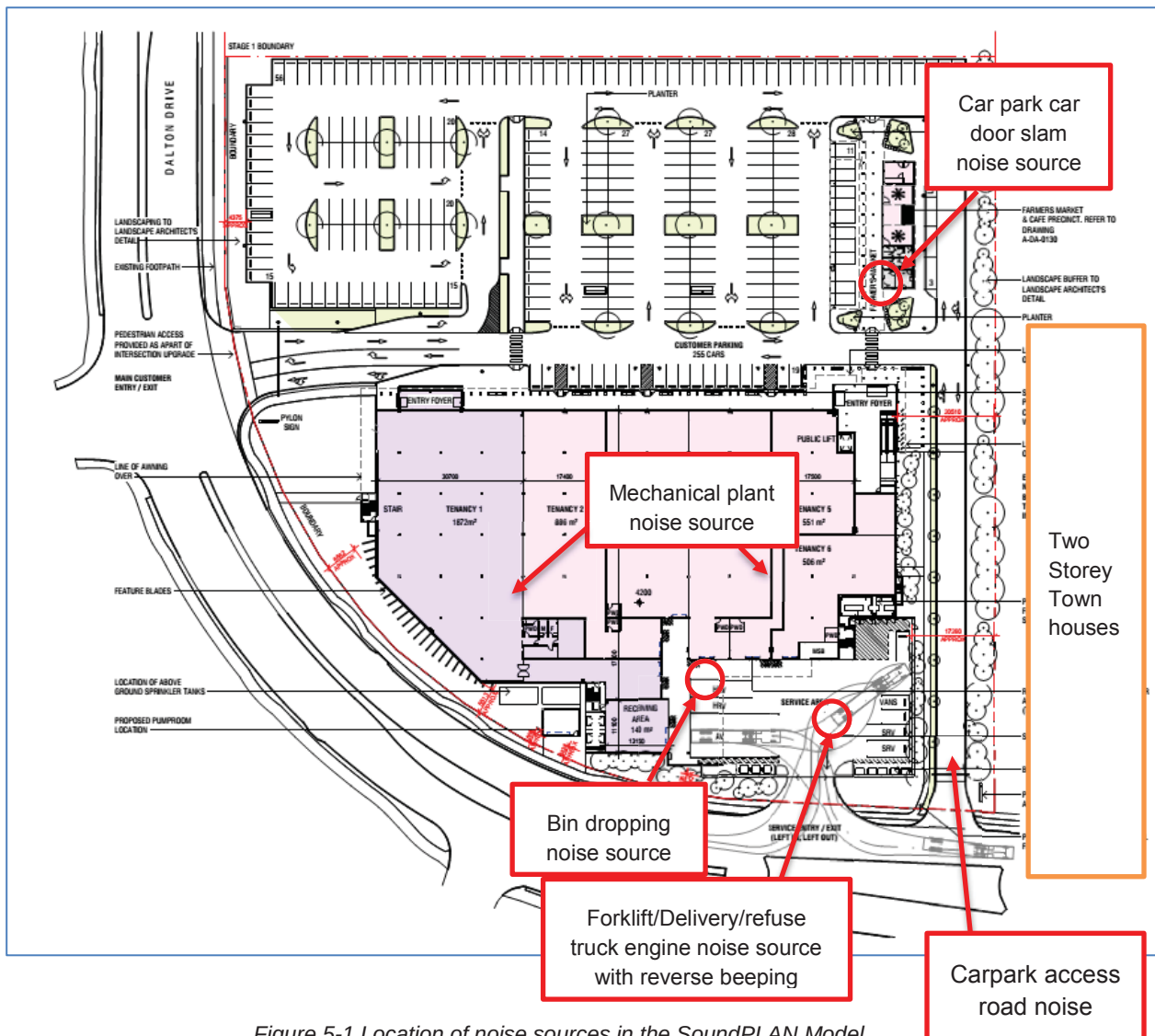
Figure 5-1 Location of noise sources in the SoundPLAN Model
