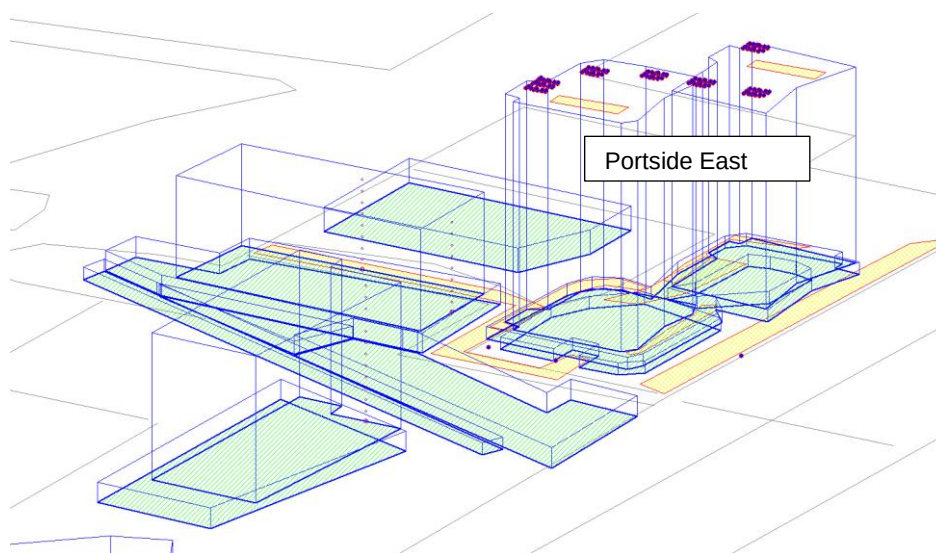
Figure 16: View of propagation model
