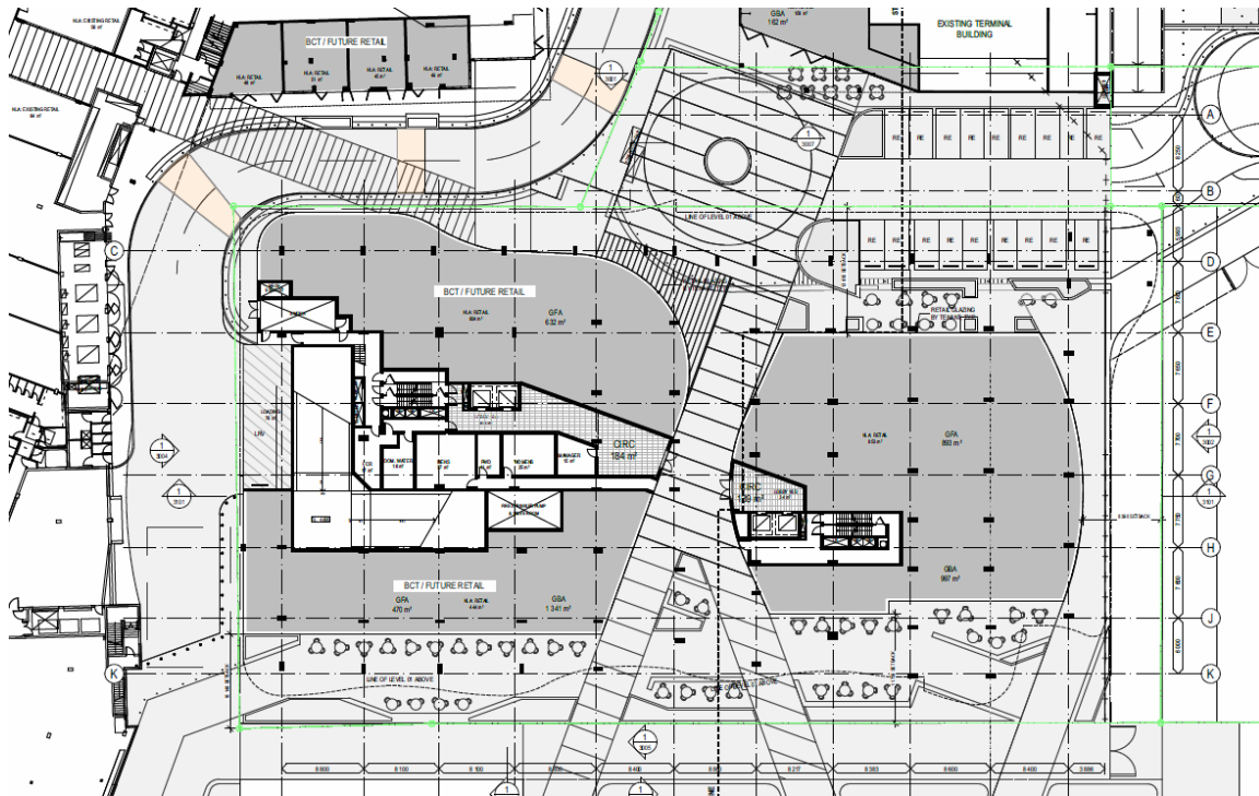
Figure 5: Extract from Drawings Showing Redeveloped Site Configuration
