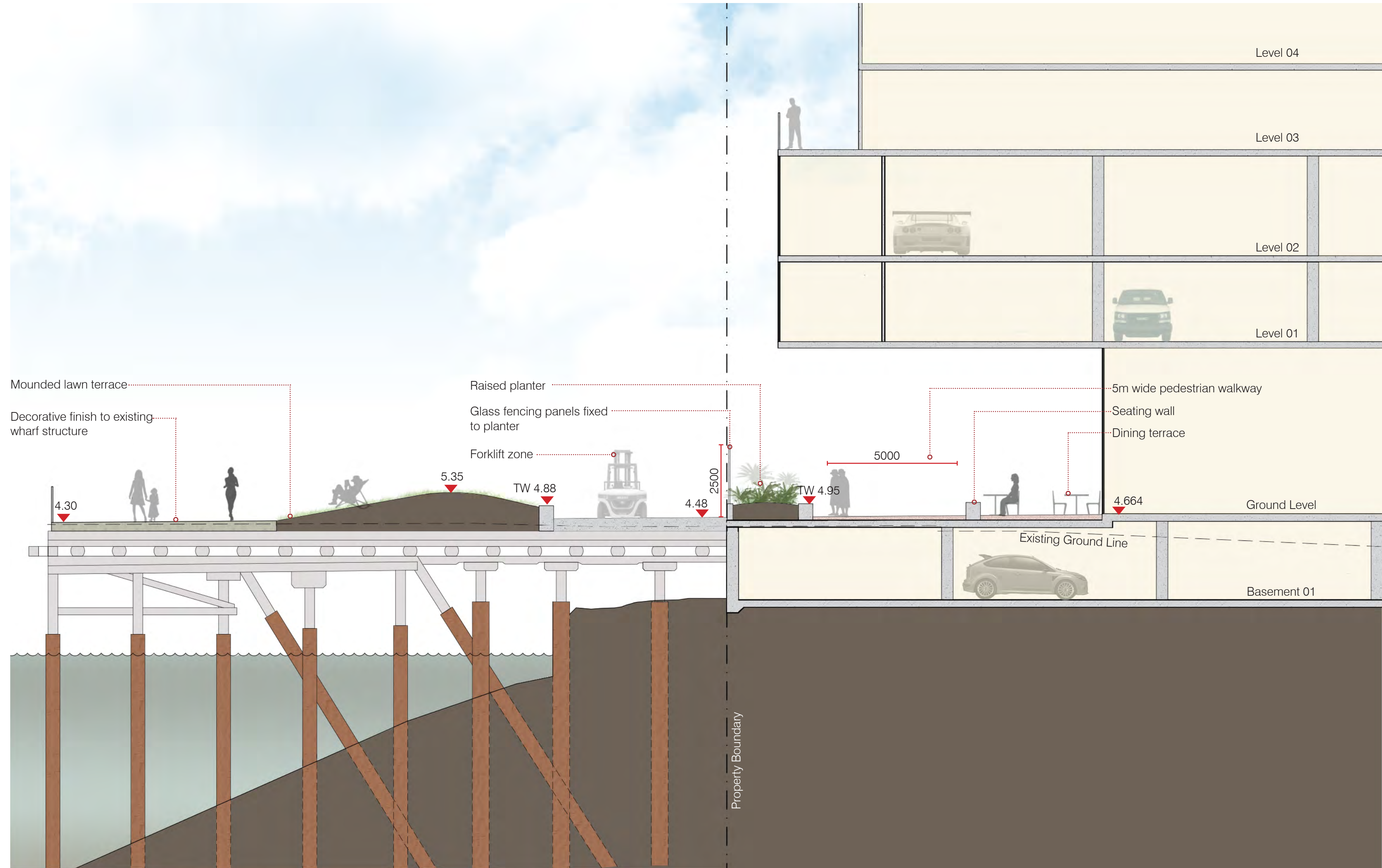
SECTION E SCALE 1:100 at A1; 1:200 at A3
