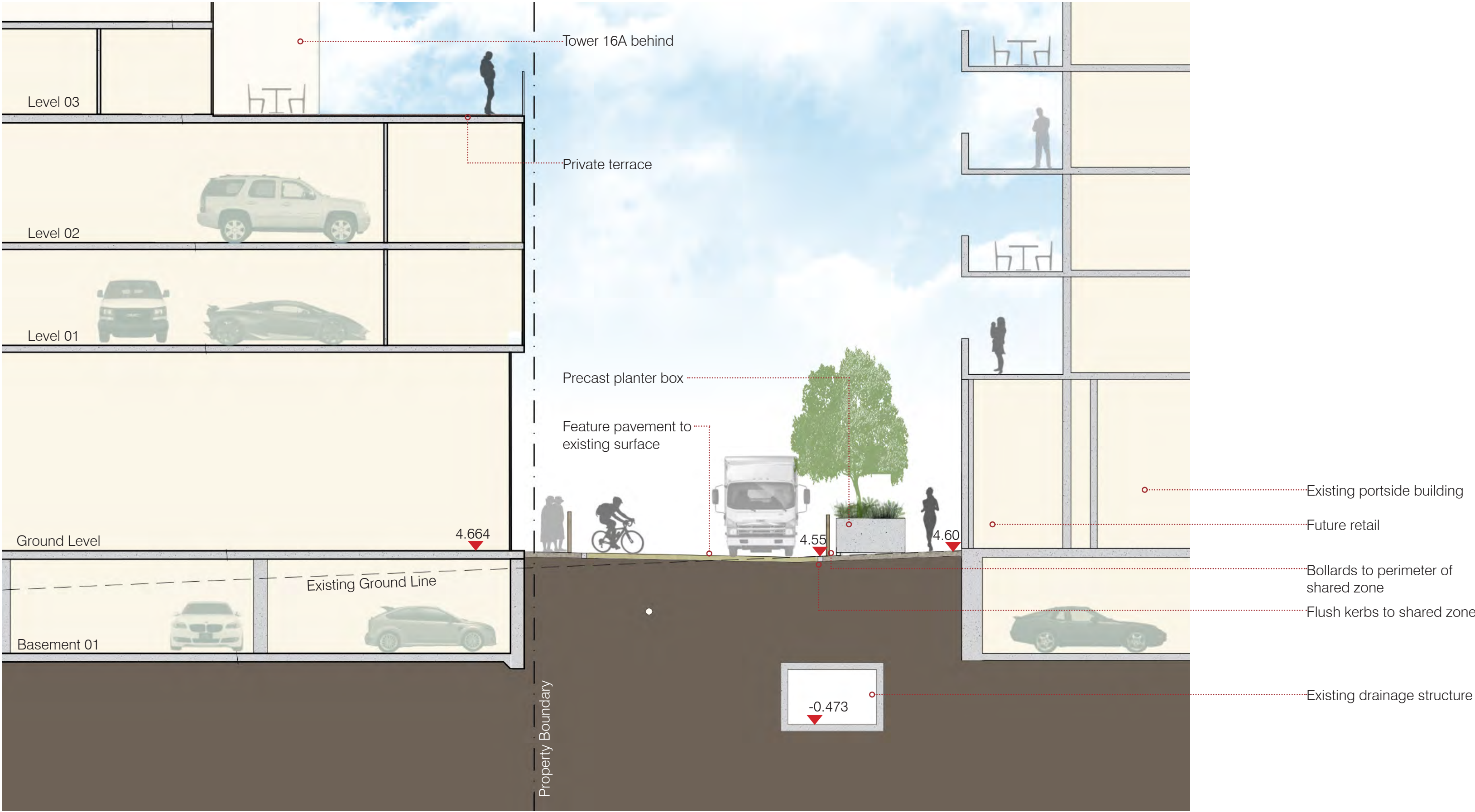
SECTION D SCALE 1:100 at A1; 1:200 at A3
