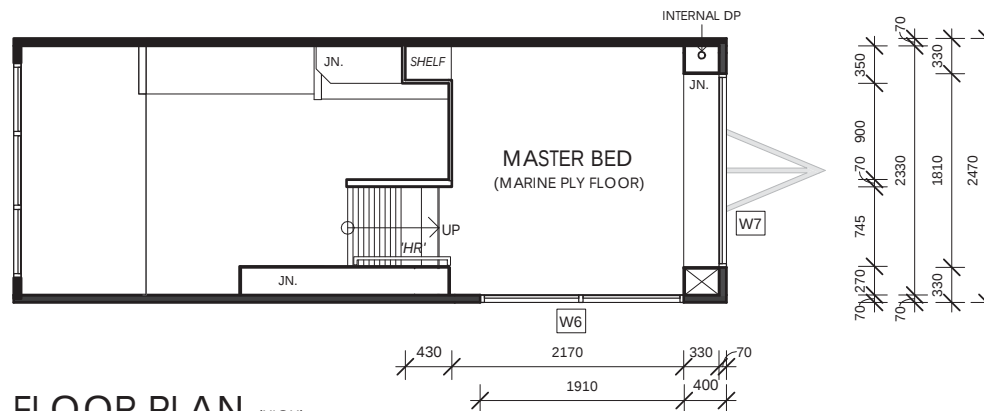
FLOOR PLAN (HIGH) SCALE 1:50
