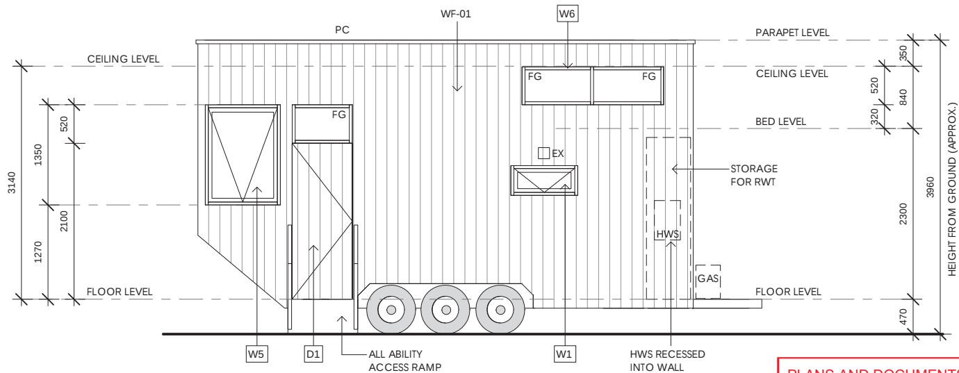
ELEVATION SIDE SCALE 1:50
