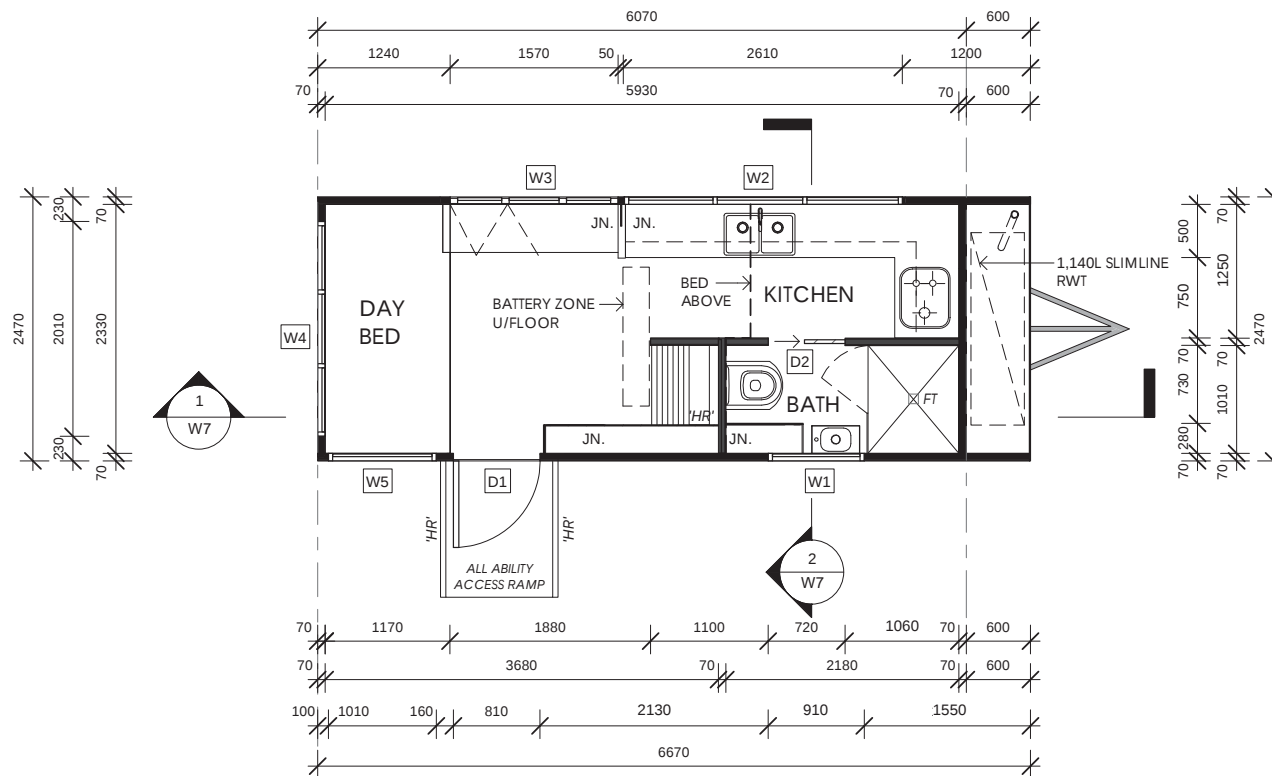
FLOOR PLAN (LOW) SCALE 1:50
