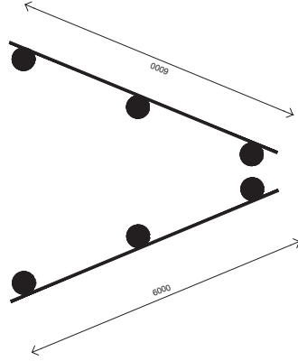
PROPOSED PLAN VIEW ON "V" SIGNS EACH PANEL 3M X 6M X 2.4M OFF THE GROUND
