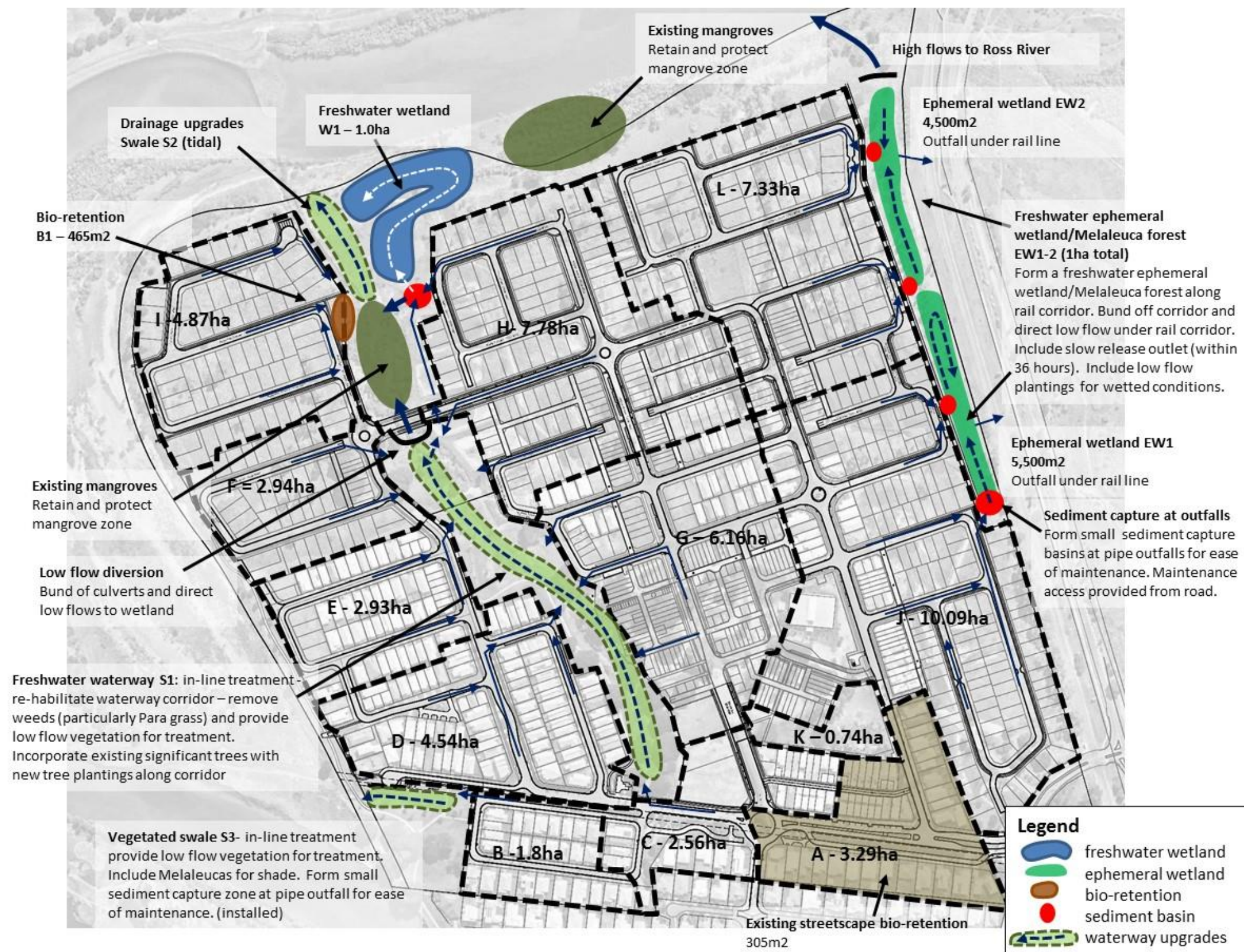
Figure 6 Ooononba stormwater treatment strategy
