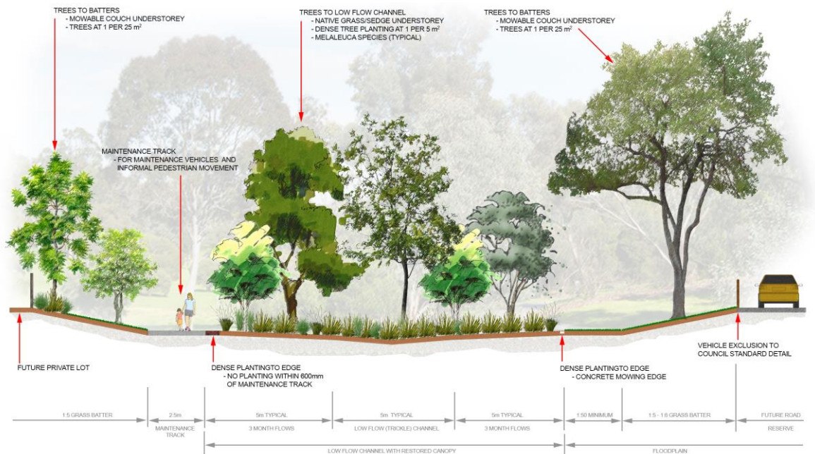
Figure 7 Typical section of a naturalised waterway
