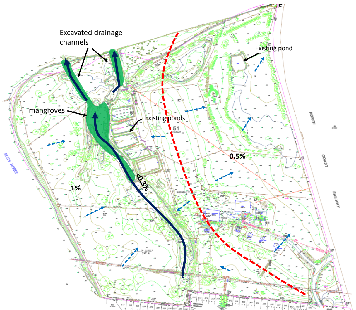
Figure 3 General drainage, catchments and topography
