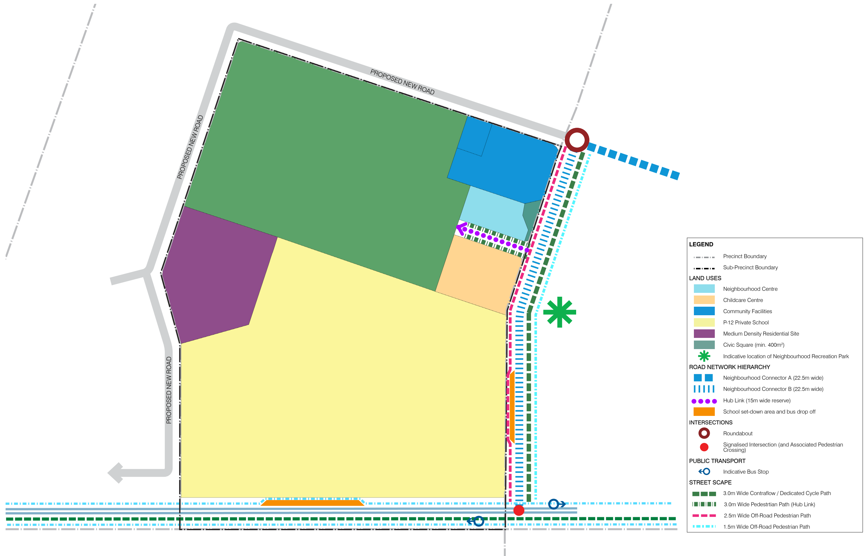
FIGURE 14: SUB-PRECINCT 12.1 FIXED ELEMENTS
