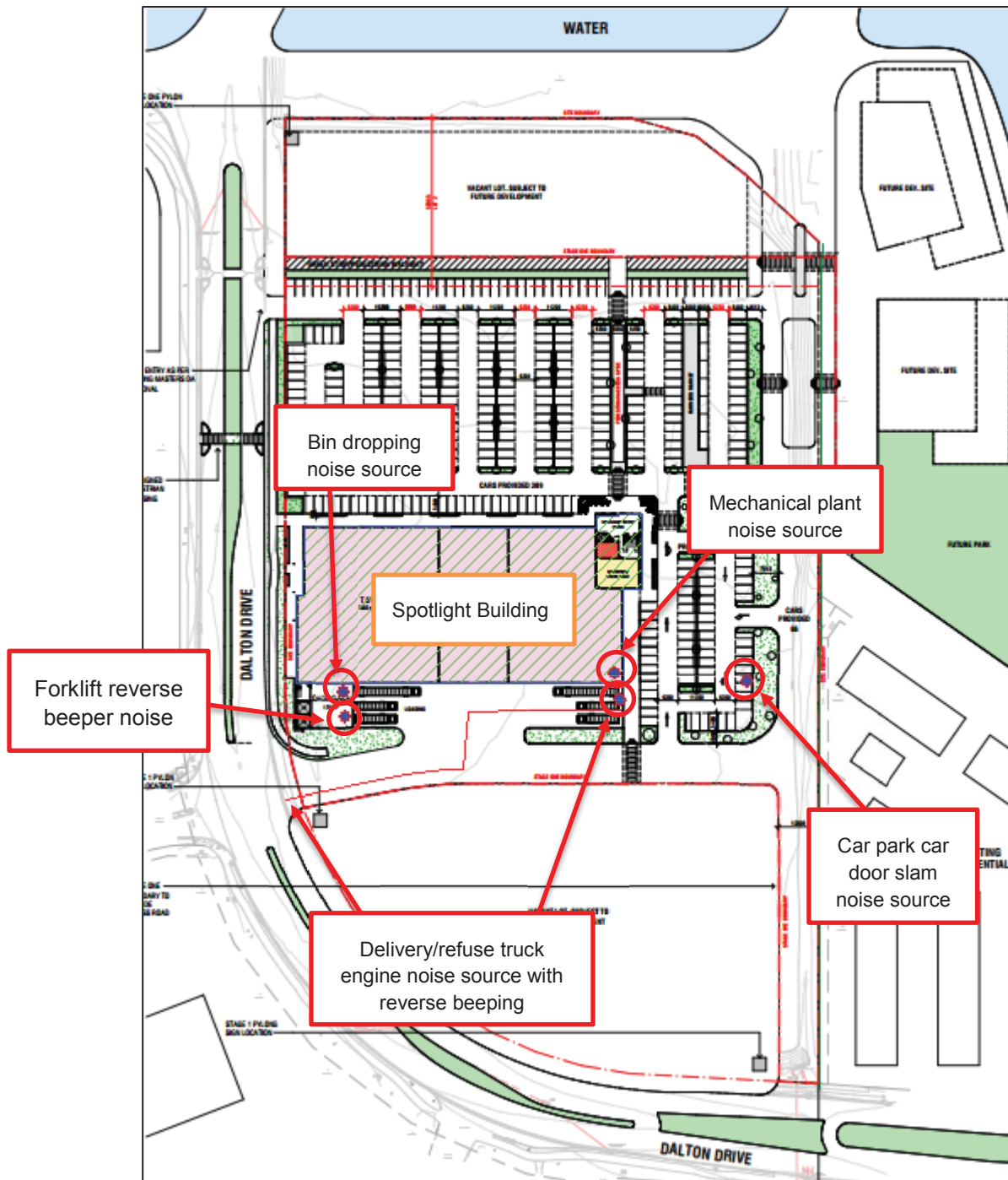
Figure 5-1: Location of the Noise Sources in the SoundPLAN Noise Model
