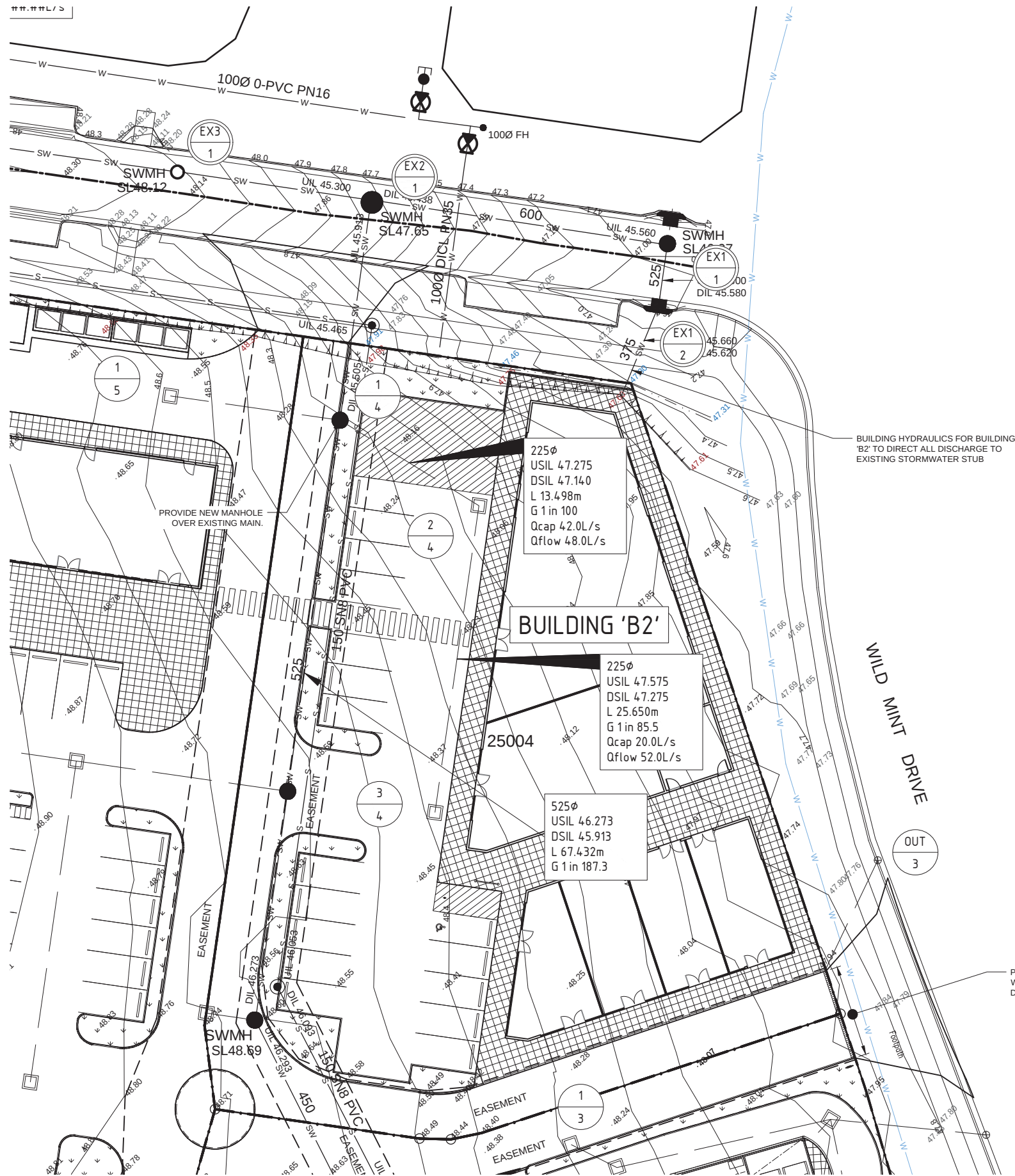
DETAIL SITE PLAN 2 SCALE 1:200
