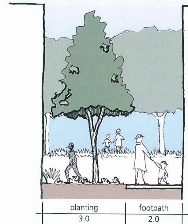
WALKWAY: SECTION D
