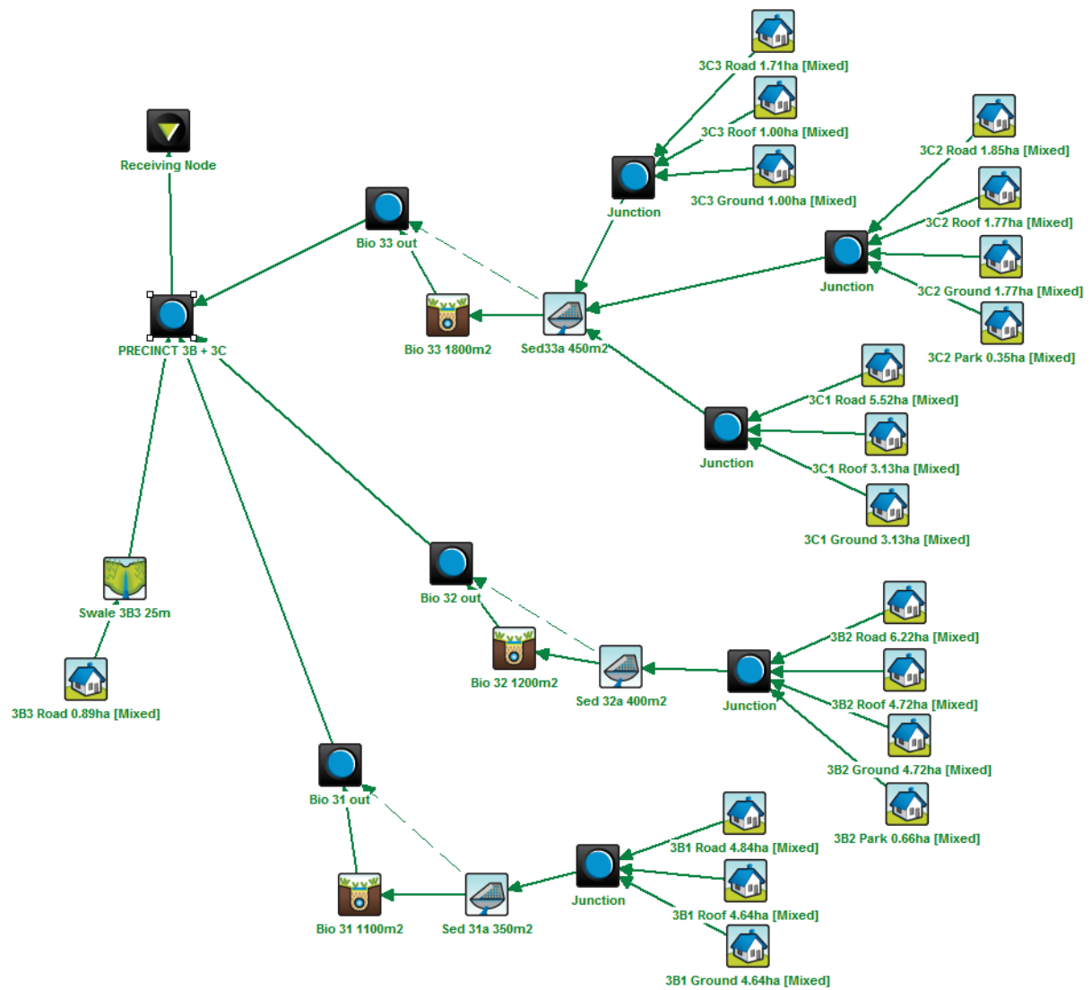
Figure 1: Precinct 3B/3C MUSIC model layout
