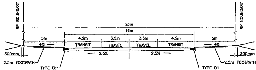
URBAN COLLECTOR ROAD - CENTRE - MULTI-MODAL - RETAIL/COMMERCIAL - SINGLE CARRIAGEWAY
