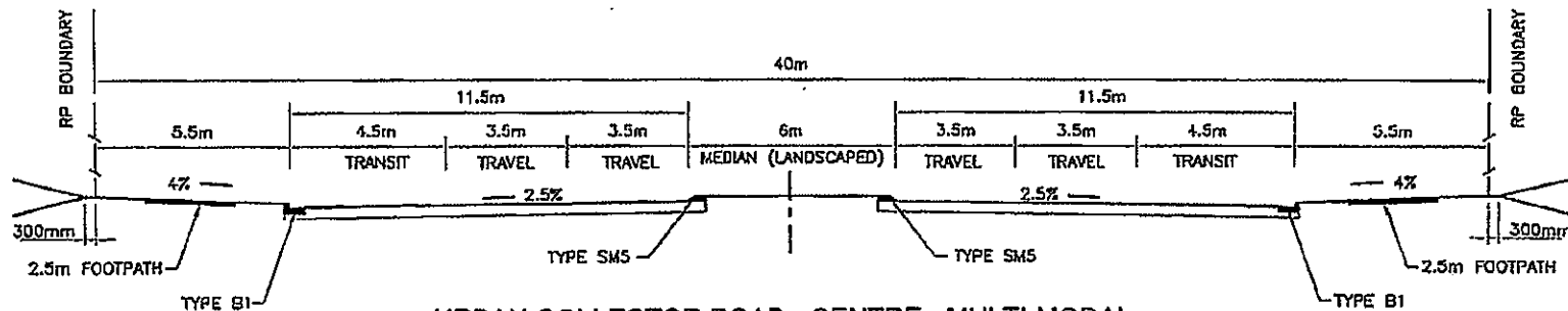
URBAN COLLECTOR ROAD - CENTRE - MULTI-MODAL - RETAIL/COMMERCIAL - FOUR LANE DUAL CARRIAGEWAY
