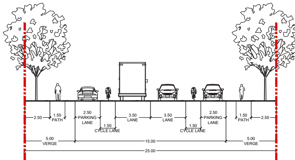
INDUSTRIAL TRUNK CONNECTOR (25m WIDE)
