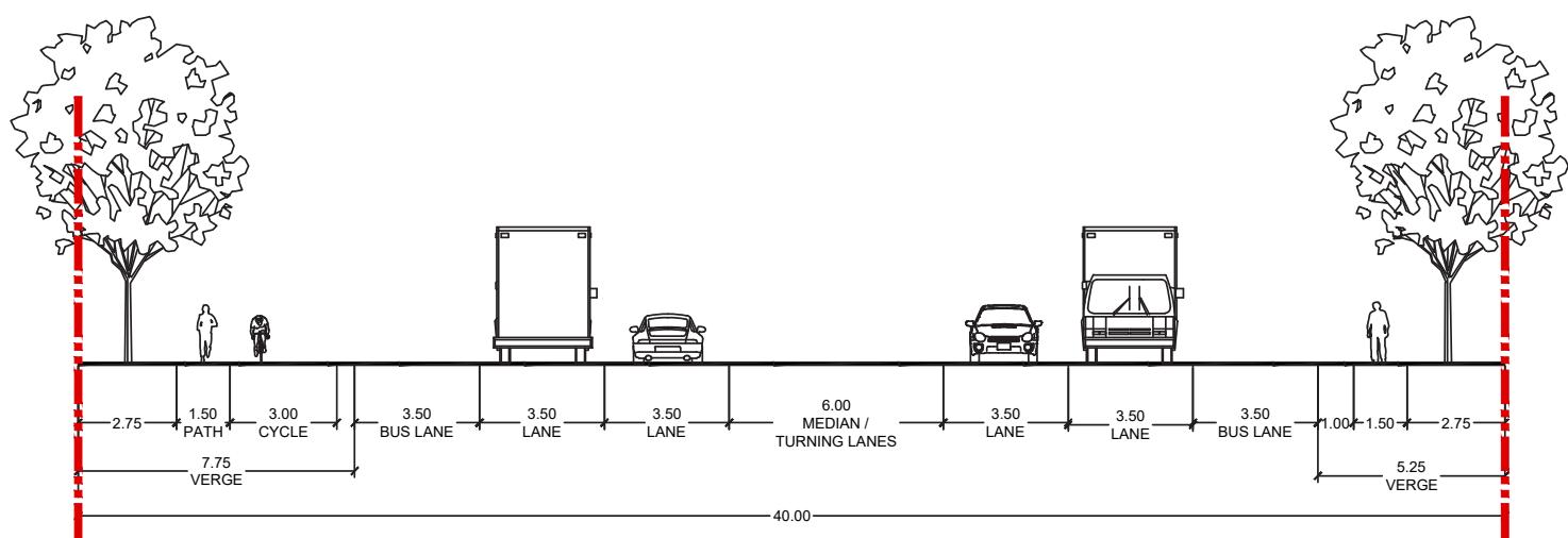
SUB-ARTERIAL - INTERSECTION (40.0m wide)
