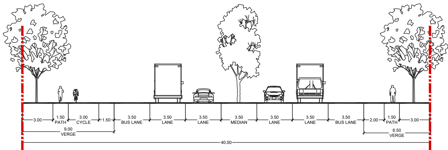
SUB-ARTERIAL - TYPICAL (40.0m wide)
